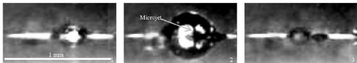
Figure 2-9. Cavitation microjet [33].
