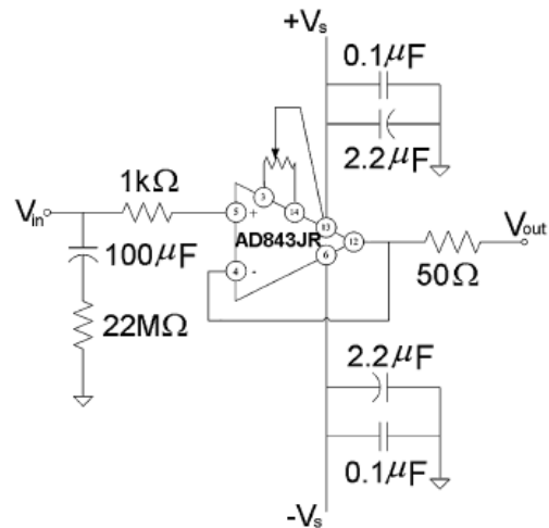
Figure 2-4 Buffer circuit [30].
