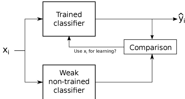
Figure 7.4: Unsupervised online-learned classifier.
