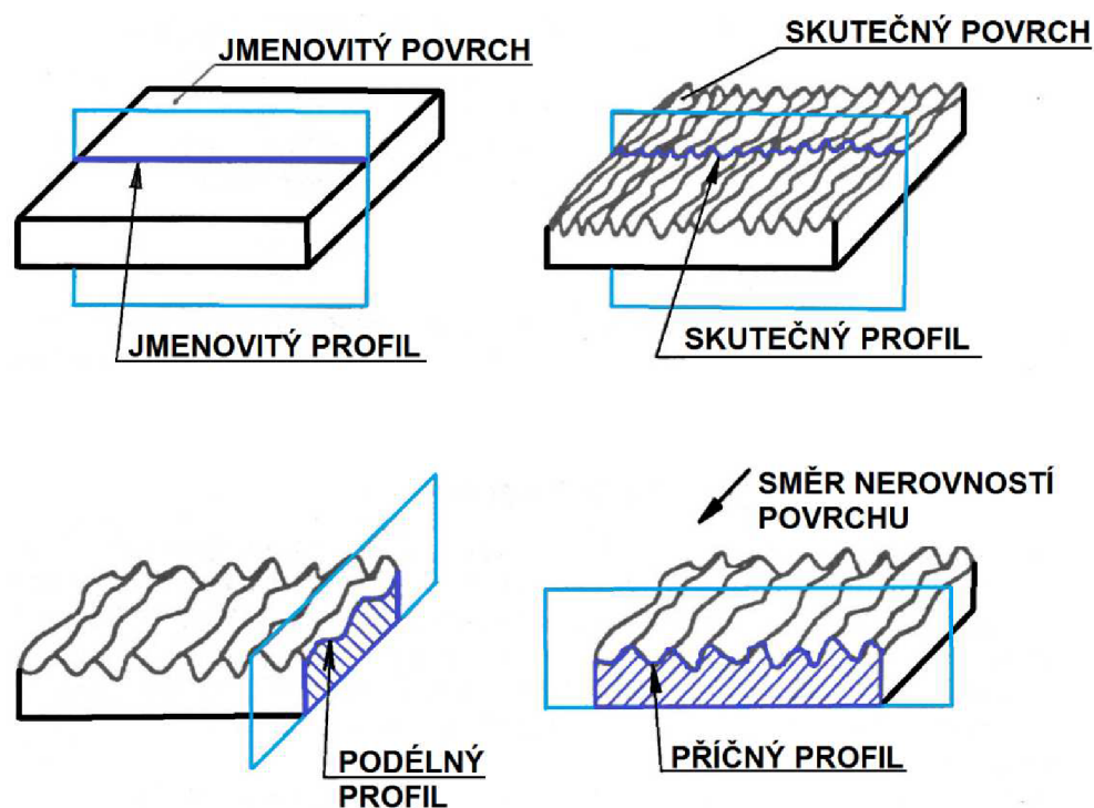
Obr. 4.8 Profily drsnosti [43]
