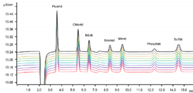
Figure 4.8: 10 chromatogram
