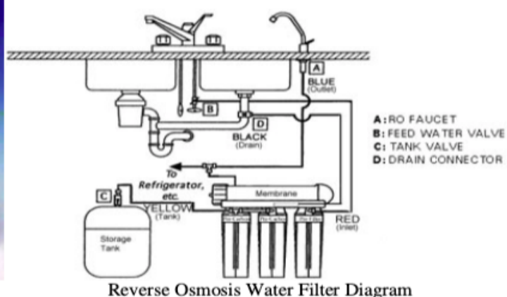
Figure 3.8: Reverse osmosis
