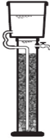
Figure 3.10: Stratified column of brick chips, pebbles and coconut shells as used in Sri Lanka.
