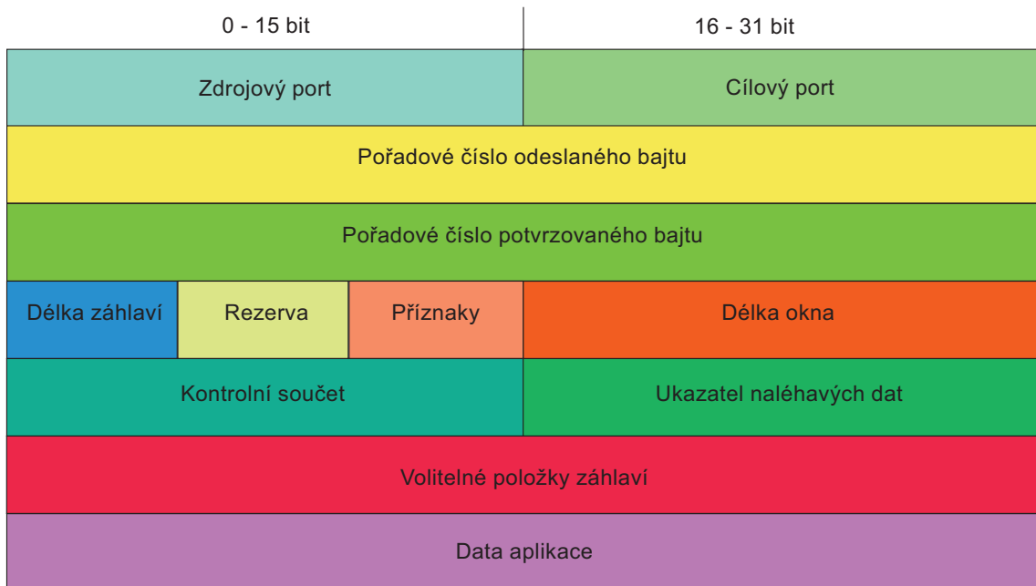
Obr. 1.12: Segment TCP.
