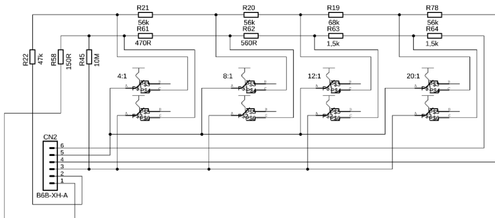
Obr. 9-13 Schéma DPS Ratio
