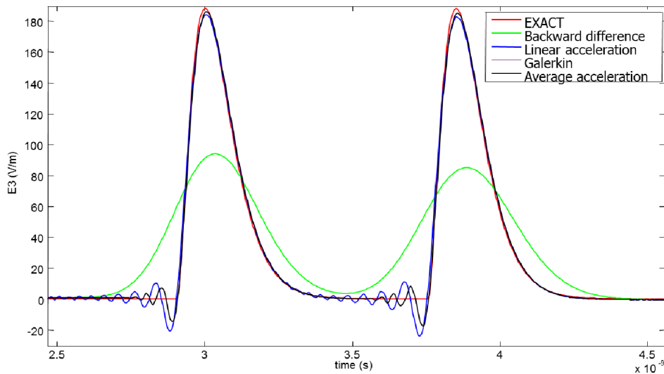
Fig. 4.5: Comparison of temporal schemes. Result after the first reflection: a sharper excitation pulse was considered.
