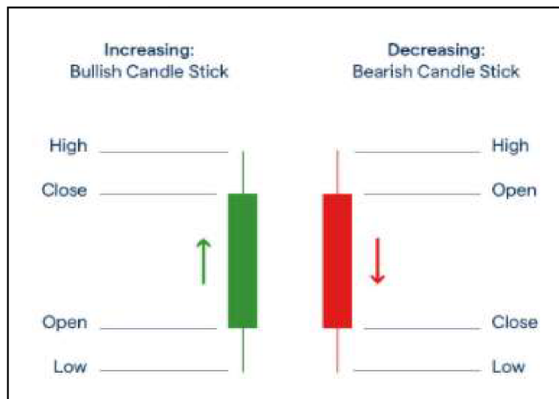
Figure 9. Candelstick Patterns
