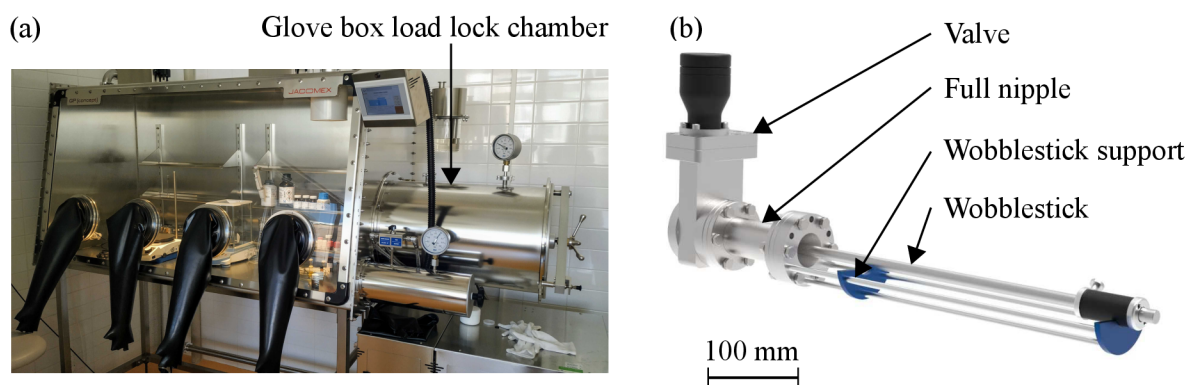
Figure 5.13: Transport extension of the atmosphere sensitive samples. (a) Glove box situated in the chemical laboratories at CEITEC. (b) Simple suitcase for transportation atmosphere sensitive samples without the pumping system.
