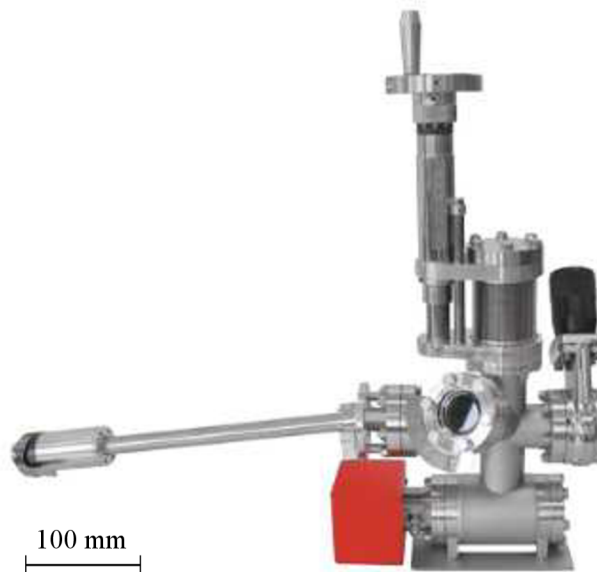
Figure 5.4: UHV suitcase from company Henniker-scientific with the linear transport sample holder up to 3 sample palette.
