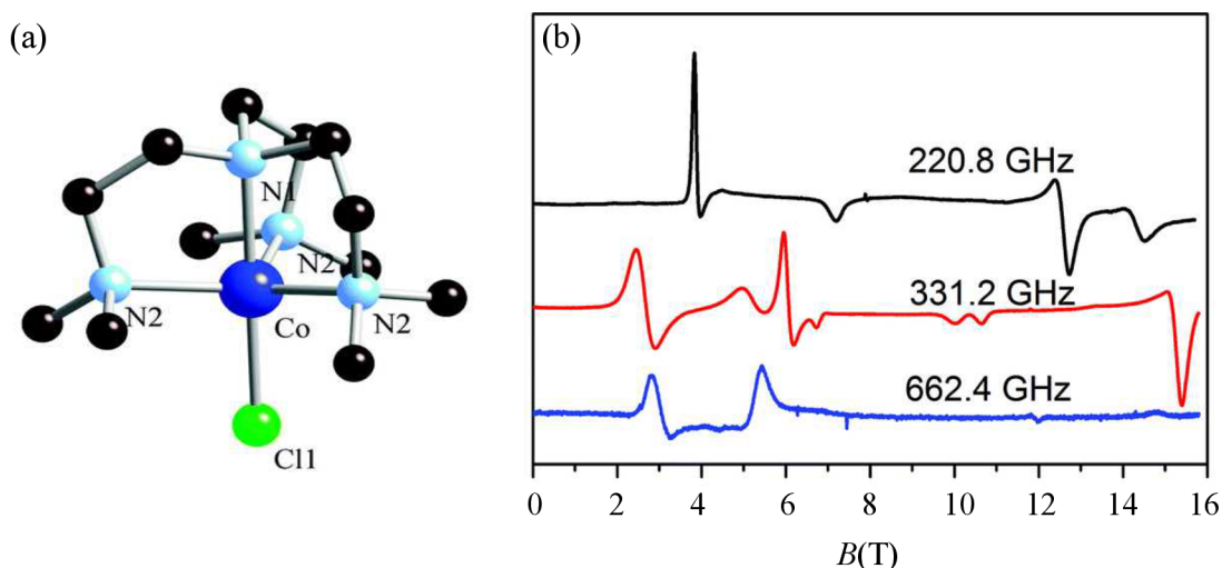
Figure 2.3: Example of molecular complex with a central transition metal ion - cobalt, (a) illustration of the molecular structure of the [\text{Co}(\text{Me}_6\text{tren})\text{Cl}]^+ (b) EPR spectrum in 220.8 GHz, 331.2 GHz and 662.4 GHz. Taken and adapted from [22].
