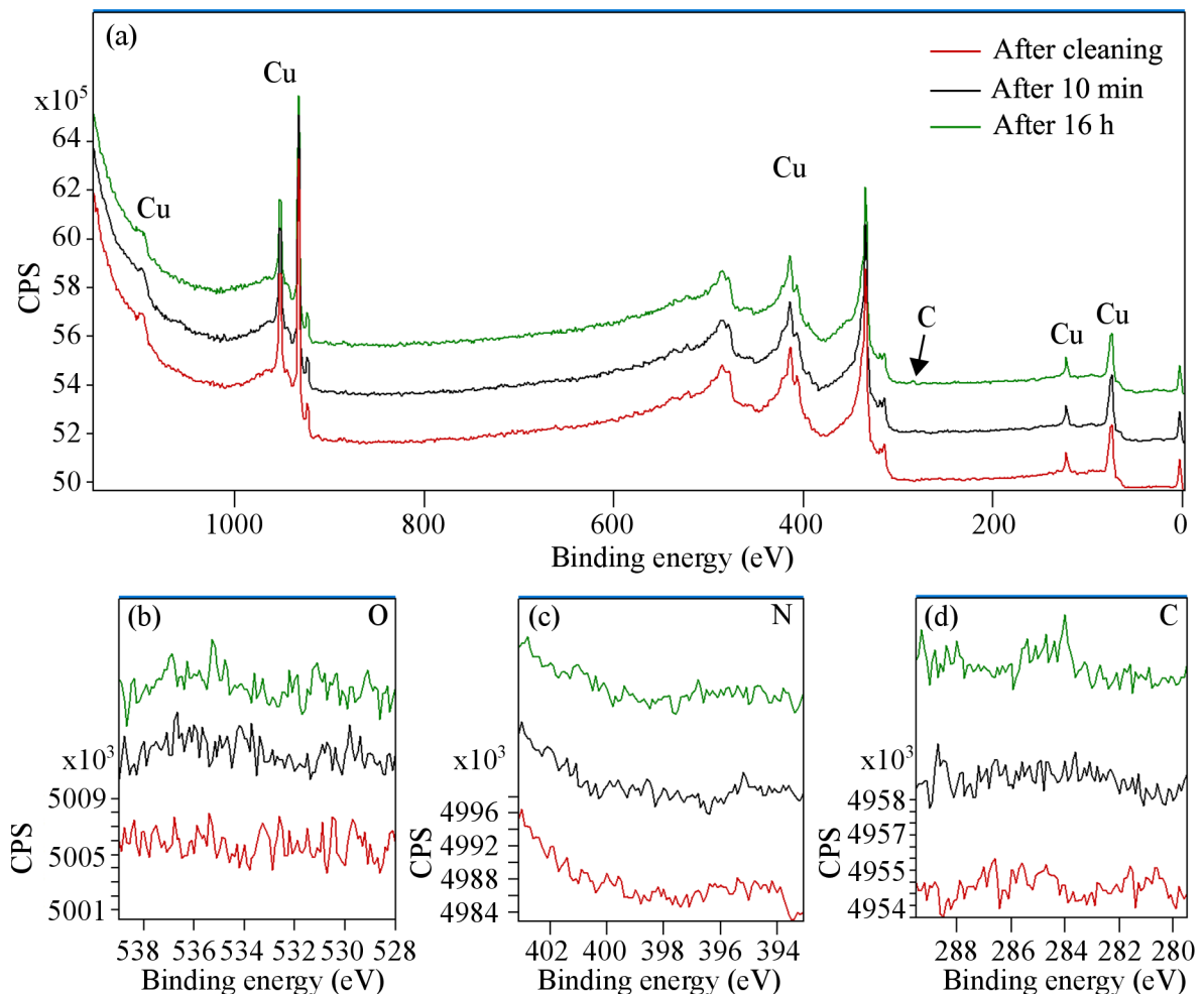
Figure 6.7: XPS spectra of Cu test sample after cleaning, 10 min and 16 h. (a) Wide spectrum of the Cu test sample. (b) Detailed measurement section for the characteristic oxygen binding energy. (c) Detailed measurement section for the characteristic nitrogen binding energy. No visible peak oxygen or carbon were displayed. (d) Detailed measurement section for the characteristic carbon binding energy.
