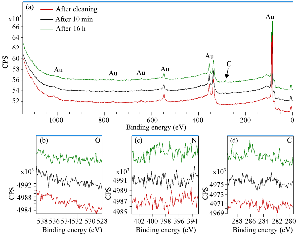
Figure 6.5: XPS characterization of the Au test sample. (a) A wide spectrum of the Au test sample. (b) Detail region, where the peak of oxygen should be observed. (c) Detail region, where the peak of nitrogen element should be observed. In (b) and (c), there can be seen just a noise. (d) Detail region, where the small peak of carbon element is observed.
