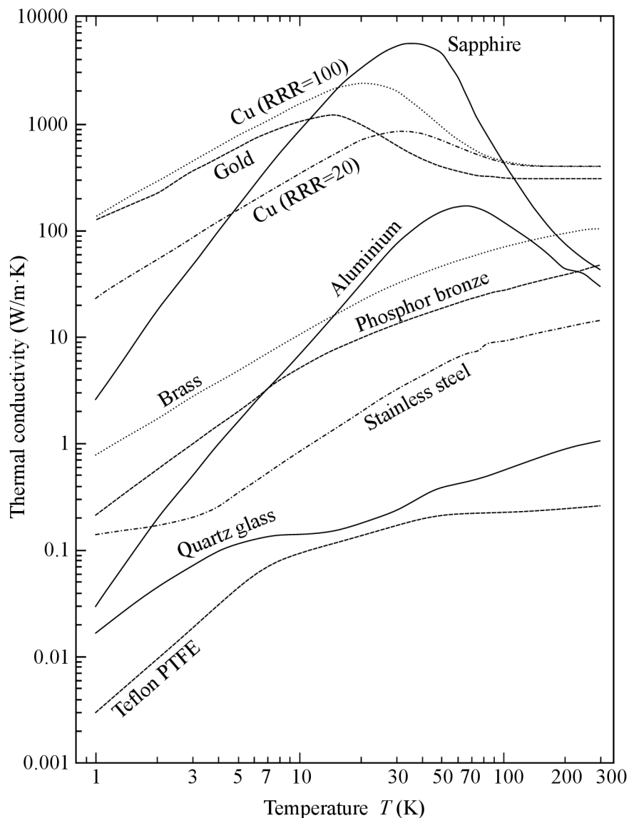
Figure 4.4: Thermal conductivity selected materials. Adapted from [68].
