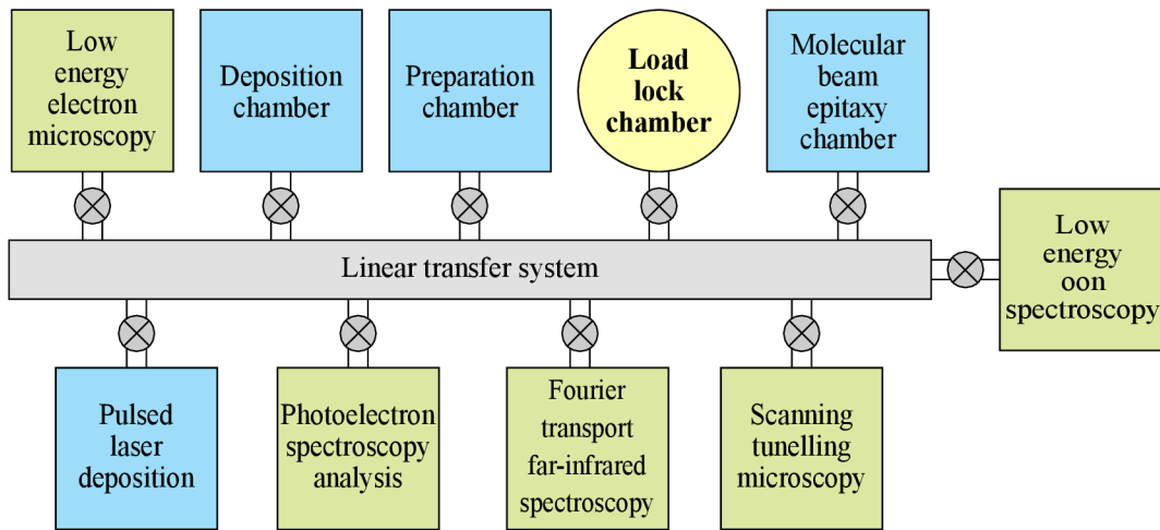
Figure 4.1: Schematic representation of the UHV cluster in the clean rooms in the institution CEITEC Nano.
