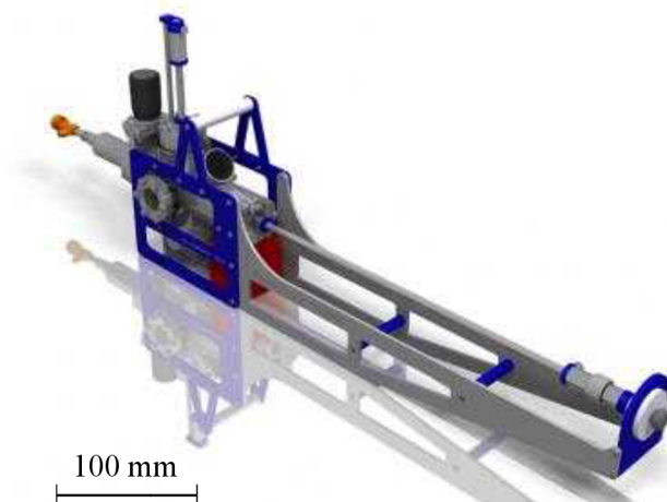
Figure 5.2: UHV Suitcase from company Ferrovac equipped with a linear transport sample storage up to three simple sample palettes.
