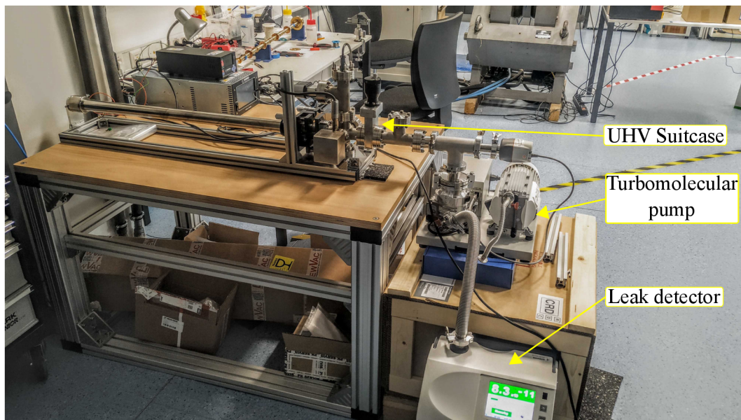
Figure 6.3: UHV suitcase connected to the turbomolecular pump with a pre-pumping leak detector. Some leaks contained in the chamber were detected using this detector.
