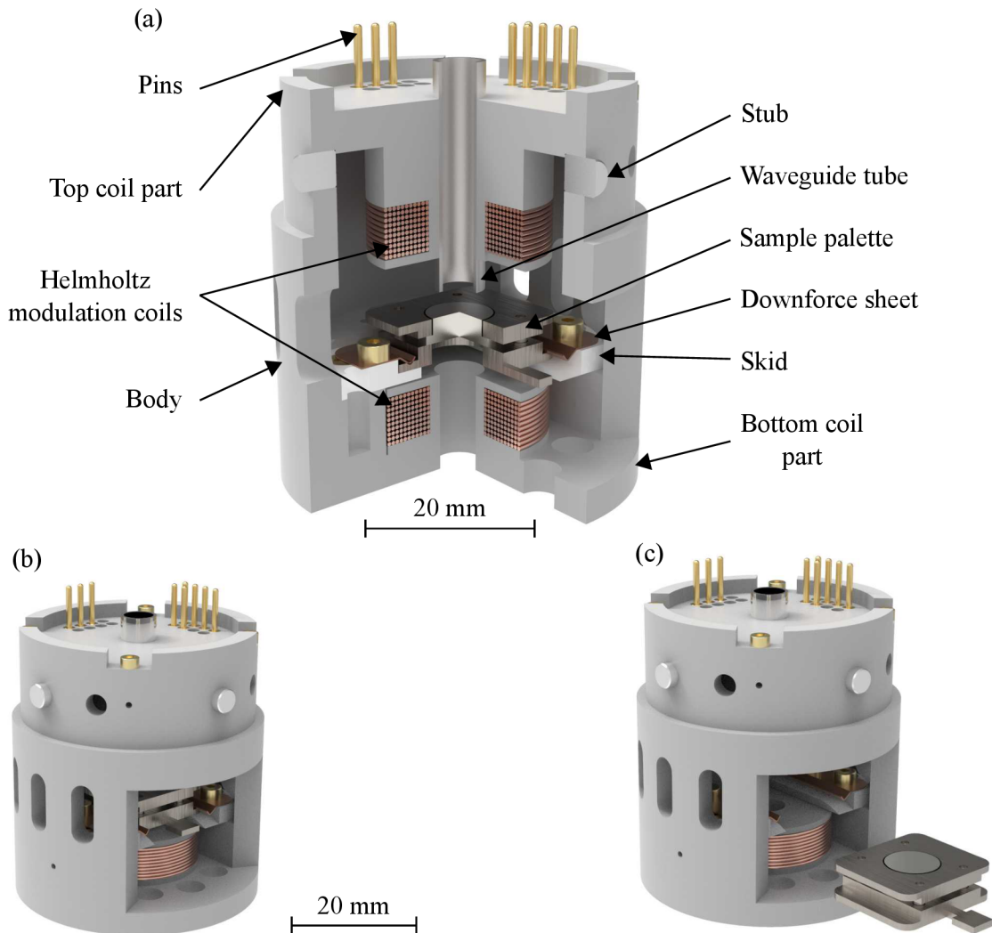
Figure 5.11: 3D model of palette holder with the sample palette. (a) Three quarter section view of the assembled palette holder. (b) View of the palette holder with inserted sample palette. (c) View of the palette holder with an ejected sample palette.
