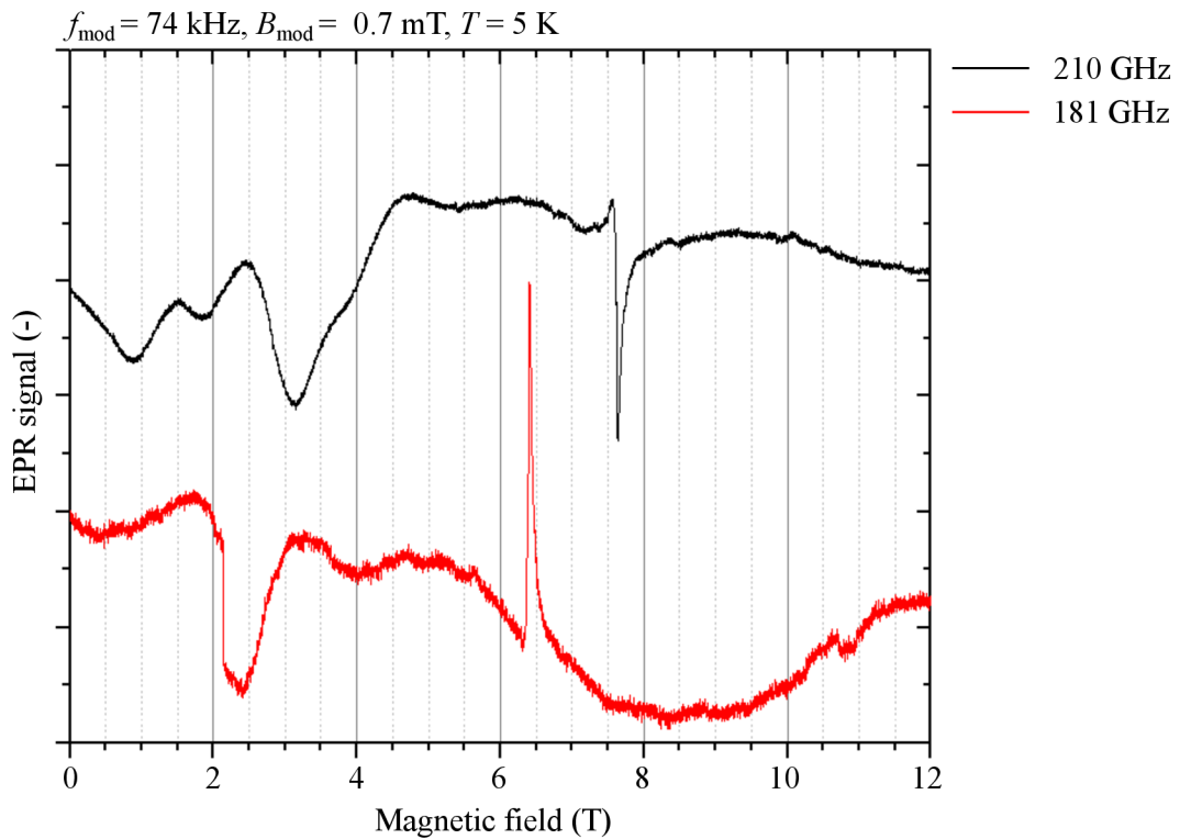
Figure 6.11: FePc reference sample in the form of the pellet. The EPR signal with the frequency 181 GHz is swept up from 0 T to 12 T, signal with the frequency 210 GHz is swept down from 12 to 0 T.
