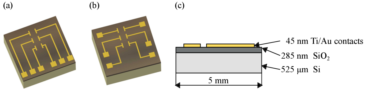
Figure 5.7: Si/SiO 2 substrates with the same size 5 mm × 5 mm include Ti/Au contacts. (a) Substrate, which is currently using for measurements graphene and its characterization. (b) Design of substrate with a more suitable placement of Ti/Au contacts for a connection with a chip expander. (c) Side view of the substrate with Ti/Au contacts.
