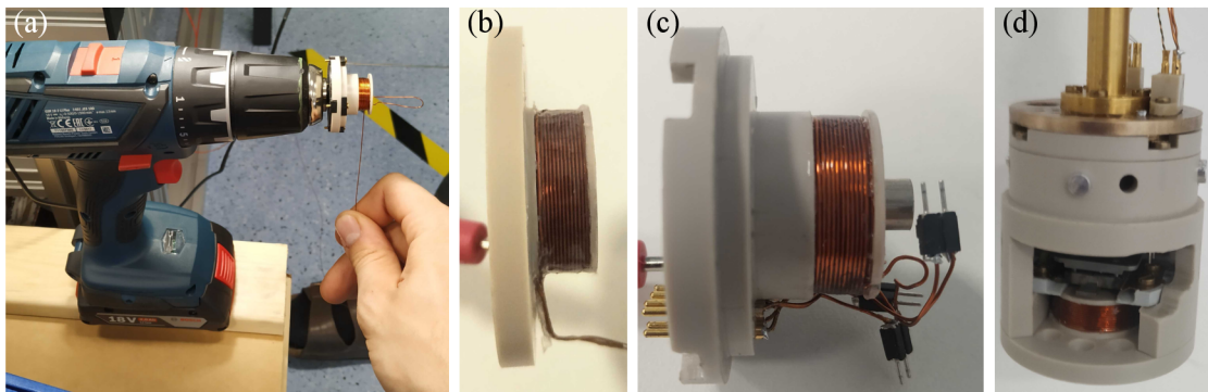
Figure A.2: (a) Method of winding coils using a cordless drill. (b) Detailed view on the bottom coil holder with wound coil. (c) Detailed view on the pincoil holder with wound coil. (d) The whole palette holder with the sample palette inside connected to the waveguide.
