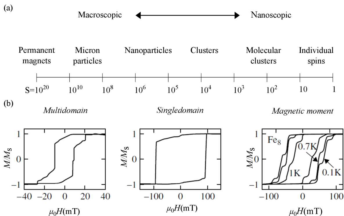
Figure 3.2: (a) overview ranging from macroscopic to microscopic scale of magnets, (b) various hysteresis dependencies of magnetization M and intensity of the magnetic field H are shown, from the multidomain through the single domain to the individual magnetic moments. Adapted from [37].
