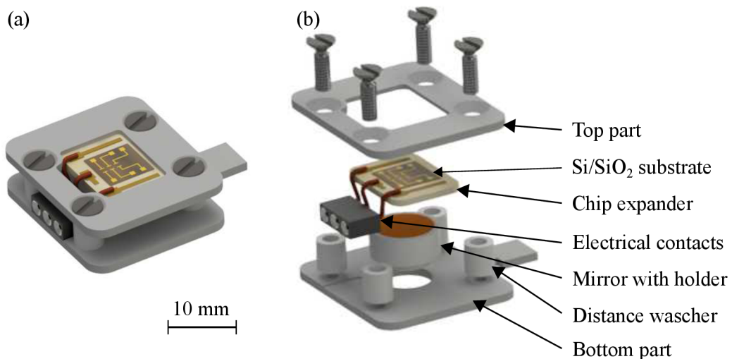
Figure 5.9: Graphene sample palette with electrical contacts. (a) Model of assembled palette. (b) Model of palette disassembled into the individual parts.
