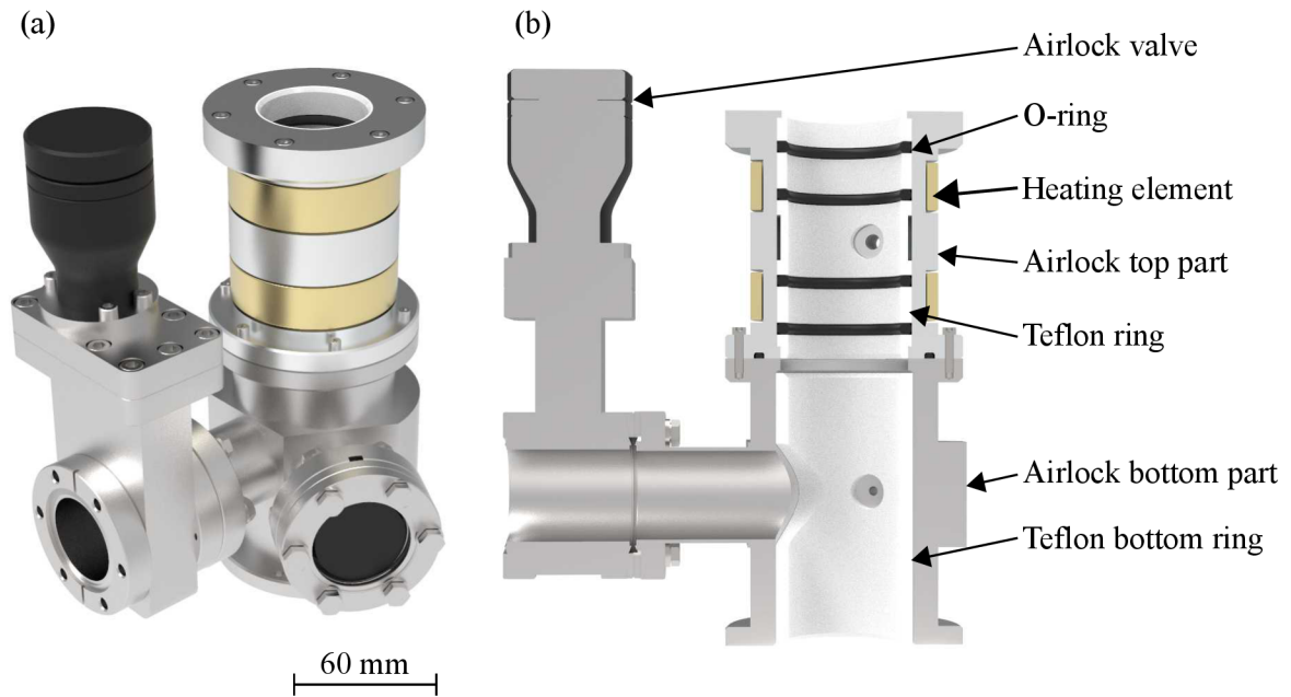
Figure 5.12: (a) 3D model of the new version of the airlock. (b) Half section view of the airlock.
