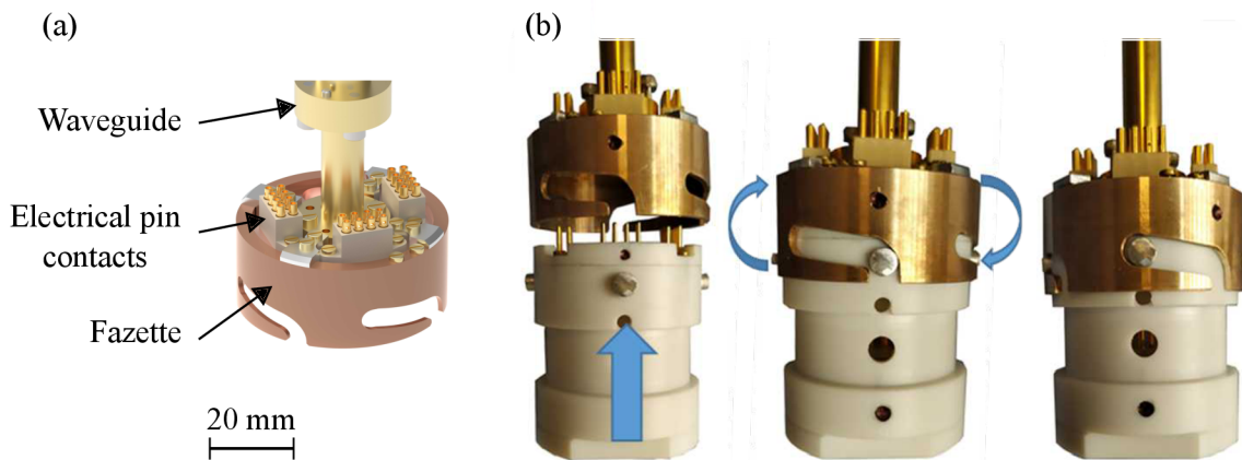
Figure 5.10: Bayonet mechanism for easy connection and disconnection of sample holders. (a) 3D model of the end of the waveguide with electrical contacts and fazette. (b) Process of mounting the sample holder to the waveguide.
