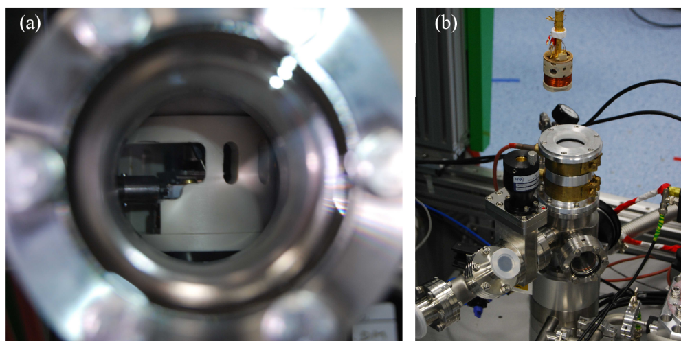
Figure 6.8: (a) Airlock inside view through the viewport. Illustration of inserting the sample palette into the palette holder by magnetic linear transfer rod. (b) Waveguide with the holder attached to the bottom inserting to the new version of the airlock.
