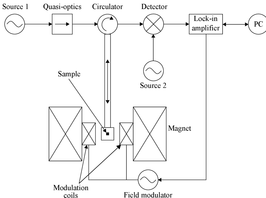
Figure 2.6: A schematic of a typical HF-EPR spectrometer with a heterodyne detection system.
