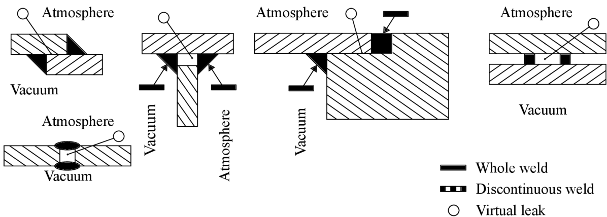
Figure 4.3: The cases of vacuum acceptable and unacceptable welds. Adapted from [60].
