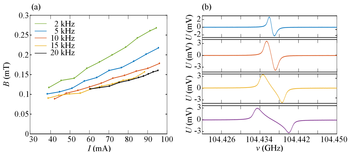
Figure 6.2: Calibration of the Helmholtz modulation coils in the palette holder inserted in the magnet. Calibration was done on the reference crystal sample of LiPc. (a) Dependence of the magnetic field in the middle of these two coils on the current flow through the coils. (b) Spectral lines of the LiPc. The input voltage from the modulation source was 9 V. The blue line has a low modulation compared to the red spectral line, which has an optimal modulation. Two spectral lines below reach the maximum amplitude (3.15 mV) of the modulation as the red spectral line, but the two peaks were begun to spread. It means that these two spectral lines are over-modulated, and lower resolution is achieved.
