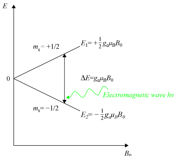
Figure 2.4: Scheme of energy-level diagram for free electron with a spin s = \pm 1/2 as a function of applied magnetic field B_0 . E_1 and E_2 are energies corresponding to m_s = \pm 1/2 states.
