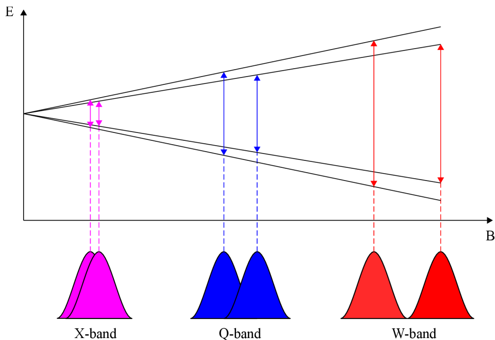
Figure 2.7: A simplified energy level diagram 2 species of different g -values. In the X-band frequency range, they are close to each other and are almost indistinguishable. After applying a higher magnetic field, the situation in the Q-band region is better, and the individual spectra can be distinguished. In the W-band frequency range are spectra fully distinguishable.
