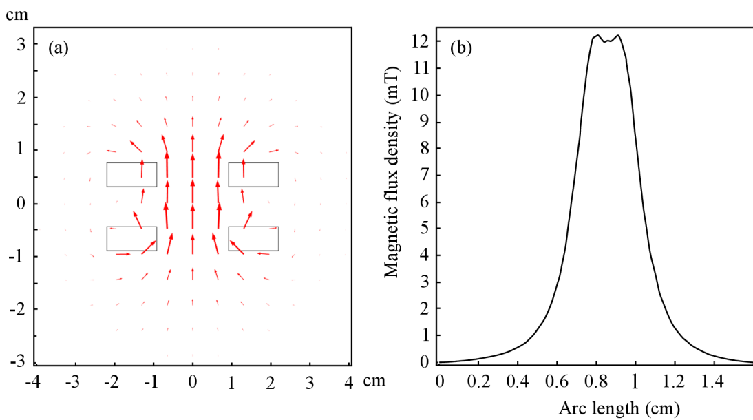
Figure A.1: Simulation of the Helmholtz modulation coils designed in thesis with a static magnetic field. Each coil has 156 turns and current I = 0.5 A. (a) Arrow surface – magnetic flux density. (b) Distribution of the magnetic flux density in the plane of the sample.
