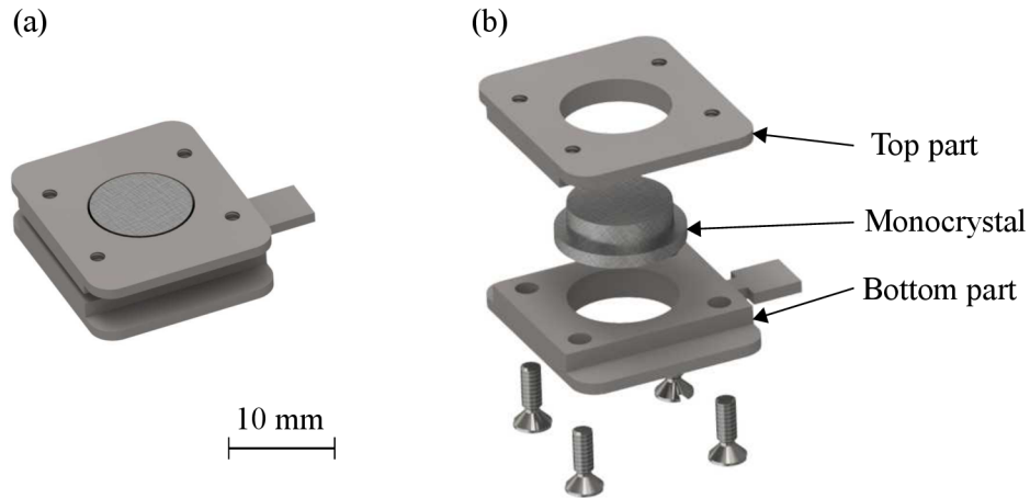
Figure 5.8: Crystal sample palette. (a) Model of assembled sample palette. (b) Sample palette disassembled into the individual parts.
