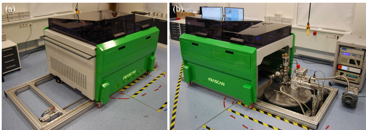
Figure 2.5: A newly-built HF-EPR spectrometer in CEITEC Nano MOTeS laboratory. (a) In the measurement position. (b) In the waveguide loading position.
