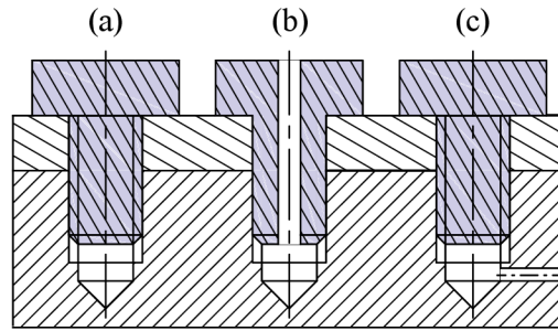
Figure 4.2: Schema of virtual leaks including: (a) the cavity under the screw, (b) the possibility to avoid the cavity by the screw with a hole, (c) by drilling the hole to the cavity from the side. Adapted from [60].
