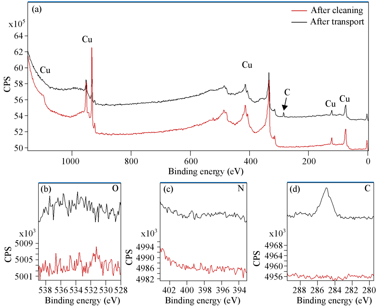
Figure 6.9: XPS spectra of the Cu test sample before and after the transport to the HF-EPR spectrometer. (a) Wide field spectrum of the Cu test sample. (b) Detail region, where the potential peak of oxygen should be observed. (c) Detail region, where the peak of nitrogen element should be observed. In (b) and (c), there can be seen just a noise. (d) Detail region, where the peak of carbon element is observed.
