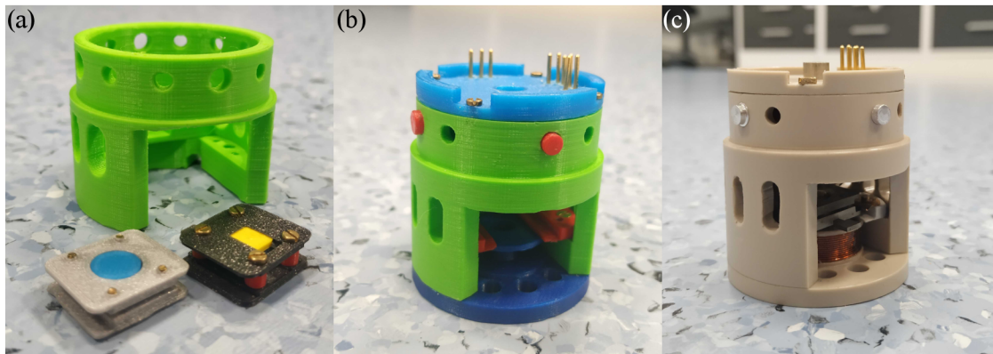
Figure 6.1: (a) First version of the palette holder with two types of sample palettes. (b) The last version of the body. 3D printed on a 3D printer Prusa MK3S. (c) Manufactured and assembled palette holder with the inserted reference sample.
