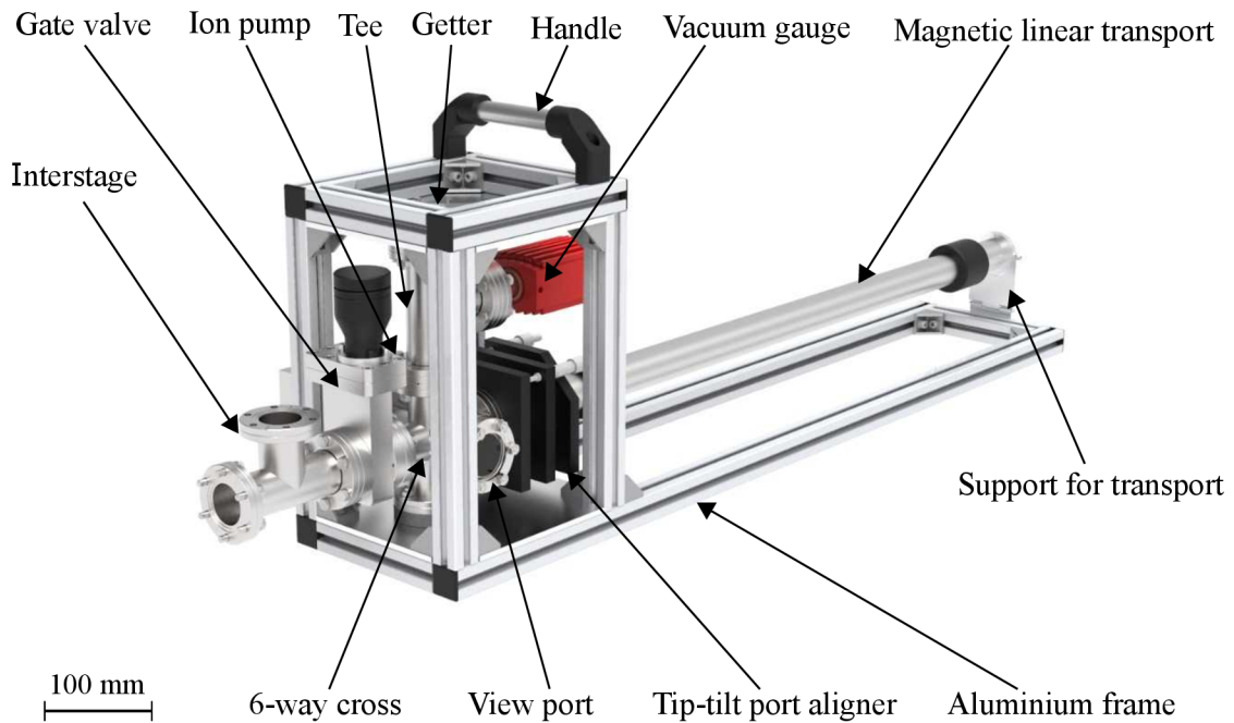
Figure 5.1: Proposed design of the mobile UHV suitcase, with indicated main parts. The overall dimensions are (412.4x276.5x1129) mm (without interstage), which allow transport of conventional personal cars trunk. The weight of 20 kg allows one person transport and operation.
