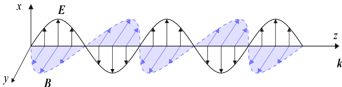
Figure 2.2: Illustration of propagating plane-polarised and monochromatic electromagnetic wave with propagation vector \mathbf{k} along z-axis.
