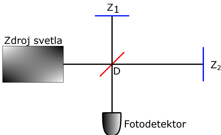
Obr. 1.10: Michelsonov interferometer
