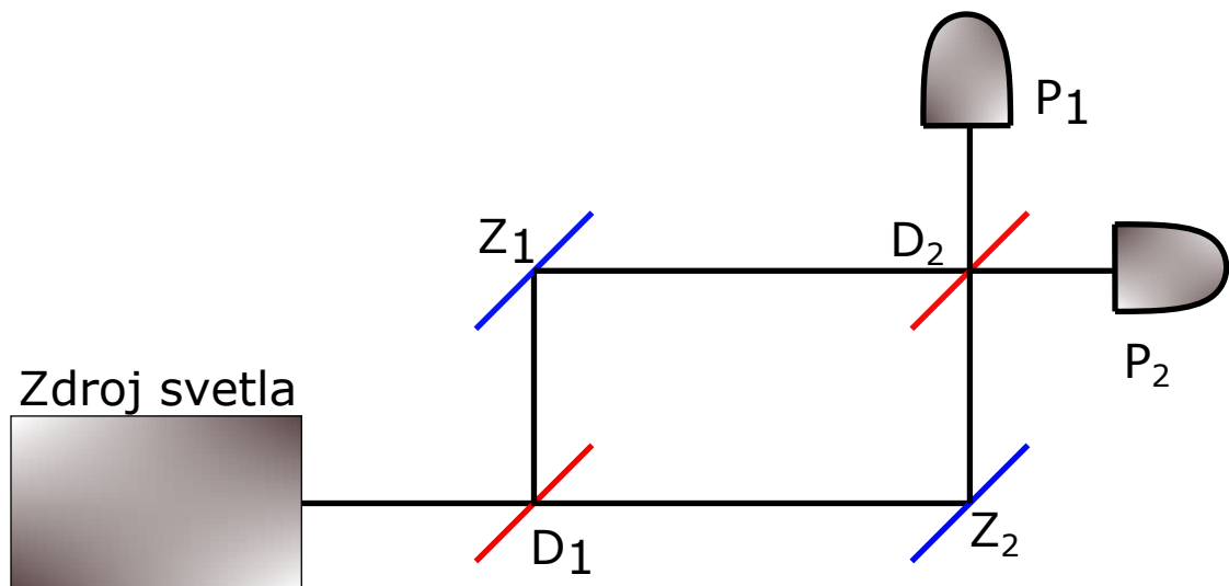
Obr. 1.8: Mach-Zehnderov interferometer
