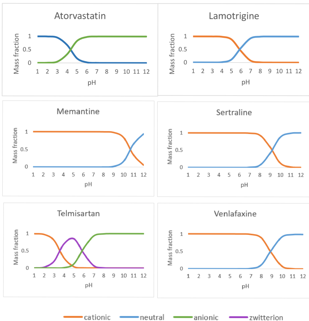
Figure 4. Mass fractions of the studied pharmaceuticals (neutral, cationic, anionic) depending on the pH of the soil.
