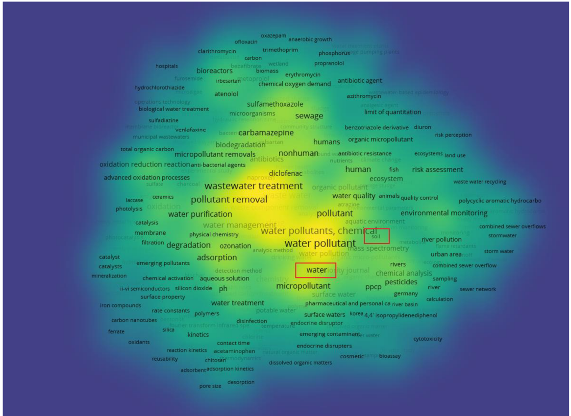
Figure 3. VOSviewer visualization of the density of key words occurrence based on the Scopus search for “micropollutants” limited to 2019-2023 years and Environmental Sciences subject.
