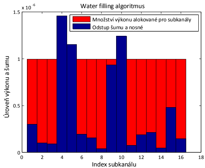
Obr. 4.3: Water filling algoritmus [42].
