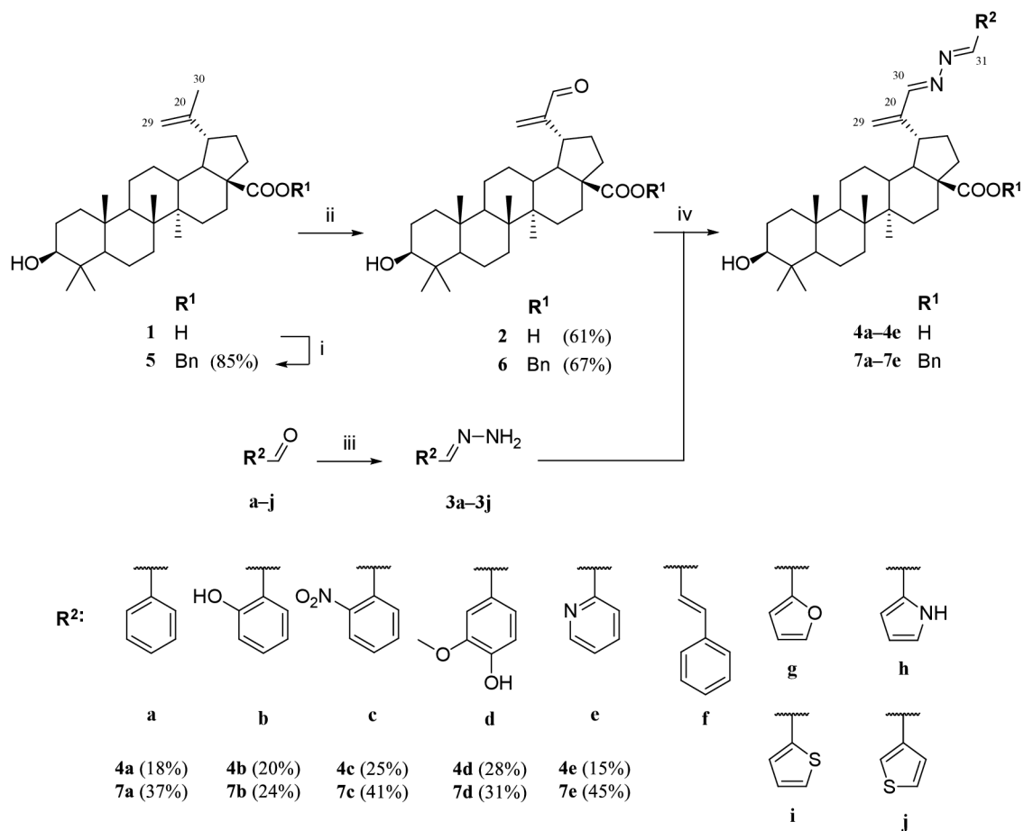
Scheme 3: Preparation of the azine derivatives 4a–4e and 7a–7e . Reagents and conditions: i) Benzyl bromide, K_2CO_3 , THF, reflux, 4 h; ii) SeO_2 , 2-methoxyethanol, 110\text{ }^\circ C , 4 h; iii) N_2H_4 \cdot H_2O , EtOH, reflux, 15 min; iv) 3a–3j or phenylhydrazine, EtOH, reflux, 2–6 h.
