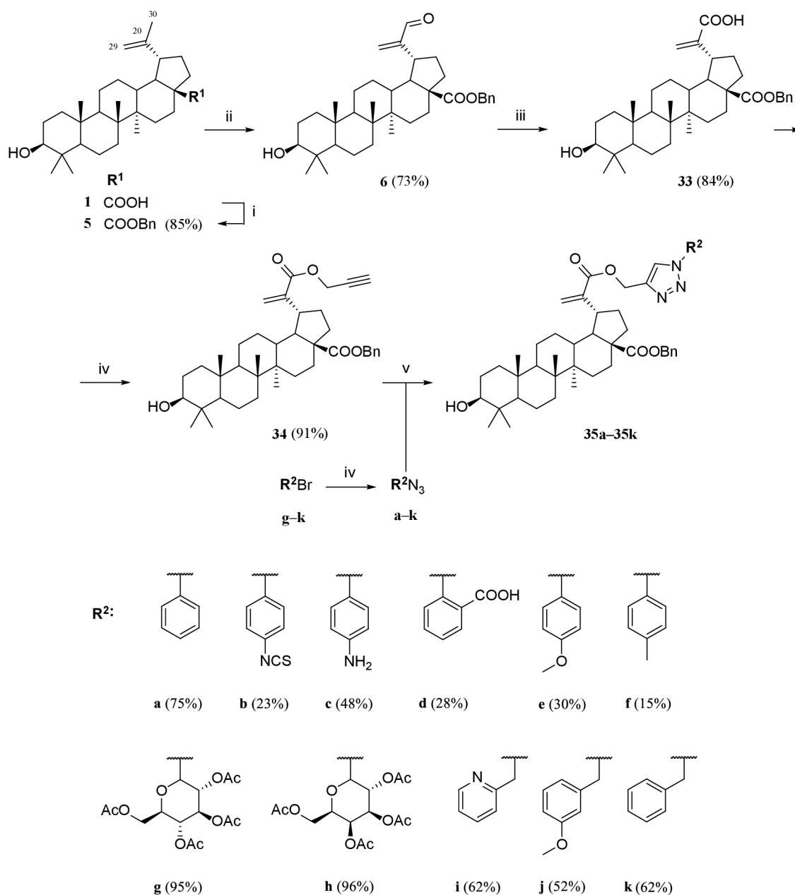
Scheme 25: CuAAC reactions on betulinic acid ( 1 ). Reagents and conditions: i) BnBr, K 2 CO 3 , THF, reflux, 3 h; ii) SeO 2 , 2-methoxyethanol, 110 °C, 4 h; iii) NaClO 2 , KH 2 PO 4 , 2-methyl-2-butene, t -BuOH/H 2 O 1 : 1, r. t. 5 h; iv) propargyl bromide, K 2 CO 3 , THF, reflux, 4 h; v) corresponding azide, CuSO 4 · 5H 2 O, sodium ascorbate, t -BuOH/H 2 O 2 : 1, 50 °C, 18 h; iv) NaN 3 , DMF, r. t., overnight.
