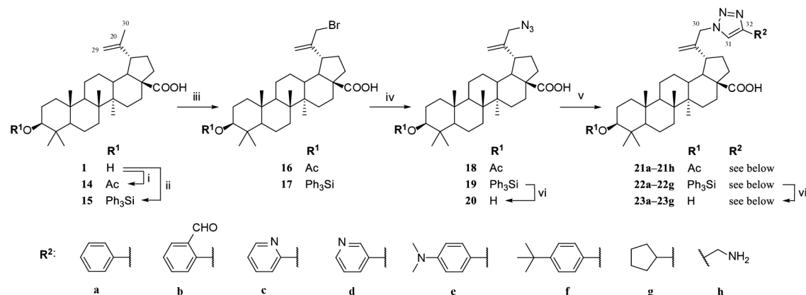
Scheme 23: Derivatives of betulinic acid ( 1 ) prepared by CuAAC reaction. Reagents and conditions: i) Ac 2 O, pyridine, r. t., 16 h; ii) Ph 3 SiCl, imidazole, DMF, r. t., 36 h; iii) NBS, AIBN, CCl 4 , 75 °C for 1 h, then 50 °C for 3 h; iv) NaN 3 , DMSO, r. t., 36 h; v) CuSO 4 · 5H 2 O, sodium L-ascorbate, alkynes a–h , DMF, r. t. or 50 °C; vi) TBAF, THF, r. t. 18–32 h, or HCl, DCM, r. t., 5–11 h. 321
