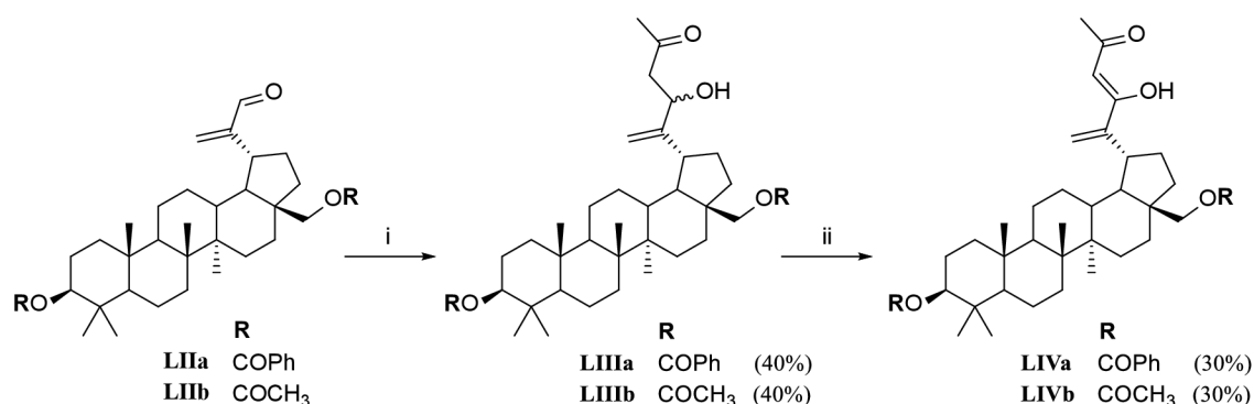
Scheme 9: C-30 derivatives prepared by Nazarov et al. Reagents and conditions: i) acetone–benzene 1 : 2, 10% NaOH, r. t.; ii) CrO 3 , H 2 SO 4 , acetone, sodium acetate, r. t., or PCC, DCM, r. t.
