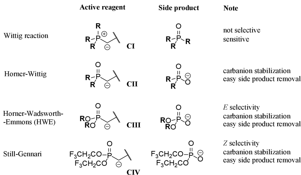
Fig. 46: Modifications of the original Wittig reaction.
