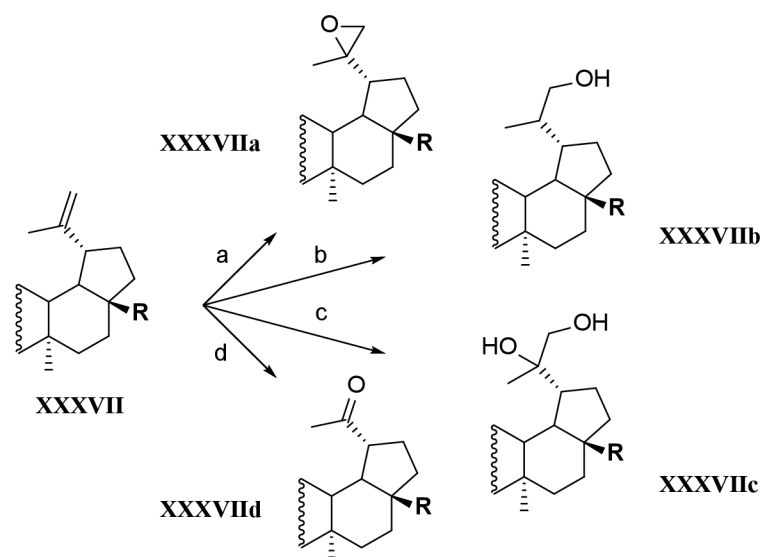
Scheme 5: Oxidation of the double bond C-20(29). Reagents and conditions: a) meta -chloroperoxybenzoic acid, DCM, 0 °C to r. t., 1 h; b) \text{BH}_3 , THF, 0 °C to r. t., 17 h; c) \text{OsO}_4 , N -methylmorpholine- N -oxide, acetone/ \text{H}_2\text{O} , r. t., 48 h; d) \text{OsO}_4/\text{NaIO}_4 , \text{MeOH}/\text{H}_2\text{O} , r. t., 20 h, or \text{O}_3/\text{Me}_2\text{S} , DCM, -78\text{ }^\circ\text{C} , 1 min.
