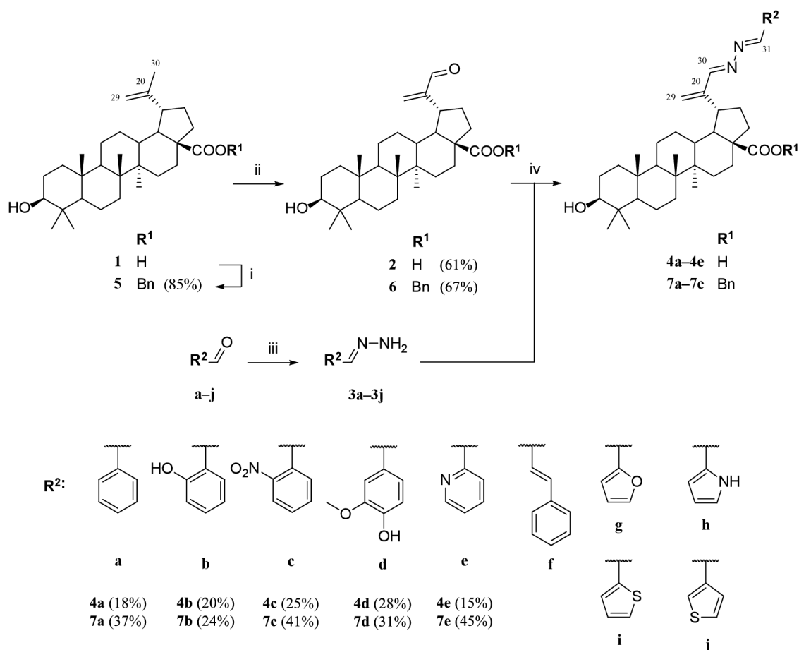
Scheme 21: Preparation of the azine derivatives 4a–4e and 7a–7e . Reagents and conditions: i) Benzyl bromide, K 2 CO 3 , THF, reflux, 4 h; ii) SeO 2 , 2-methoxyethanol, 110 °C, 4 h; iii) N 2 H 4 · H 2 O, EtOH, reflux, 15 min; iv) 3a–3j or phenylhydrazine, EtOH, reflux, 2–6 h.
