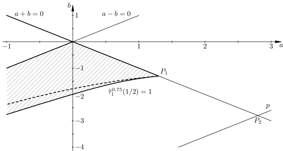
Figure 3.6: Delay-dependent parts of the stability regions \Sigma_1^{0.75}(1/2) and \Sigma_1^* for c = -0.3
