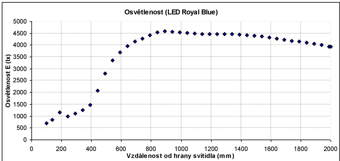
Obr. 5-12 Osvětlenost – svítidlo LED (Royal Blue LED) [18]
