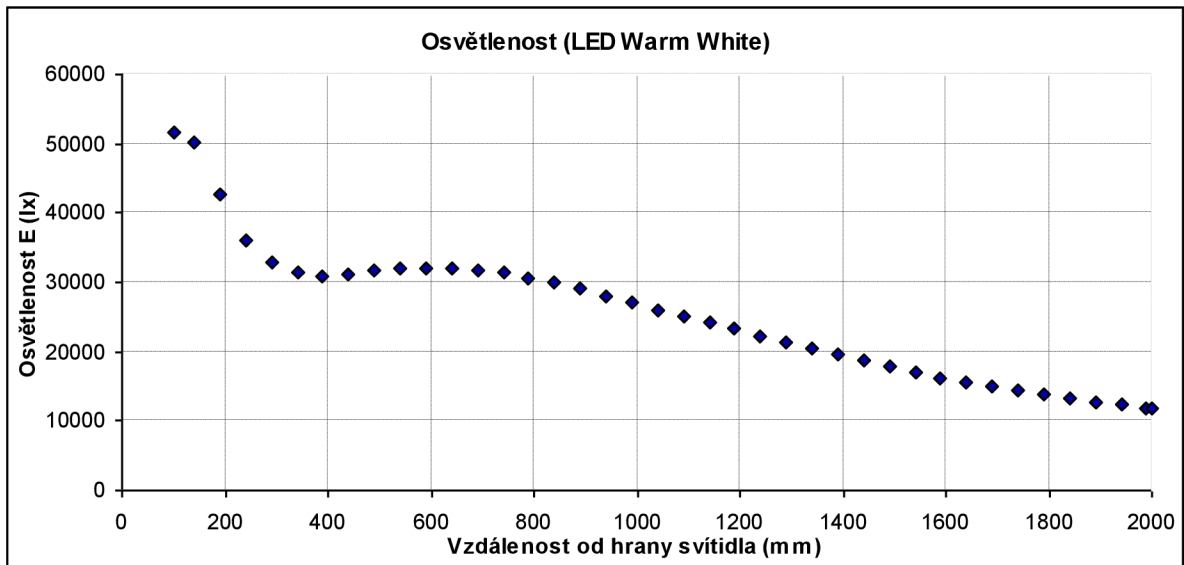
Obr. 5-11 Osvětlenost – svítidlo LED (Warm White LED) [18]
