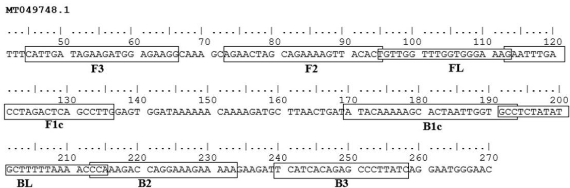
Figure 5: Position of primers on the M1 gene on IBV genome in NCBI (No. MT049748.1).
