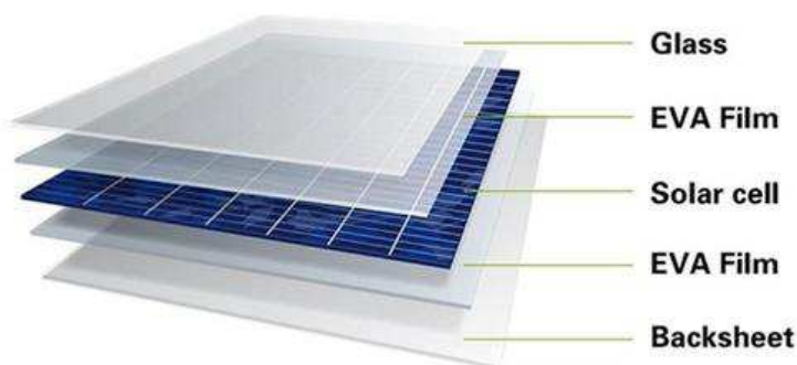
Figure 3-11 Cross section of a photovoltaic module [15]
