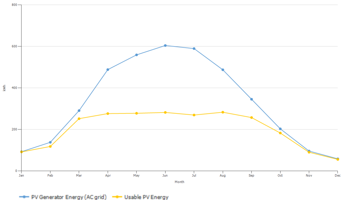
Figure 4-28 PV generated energy
