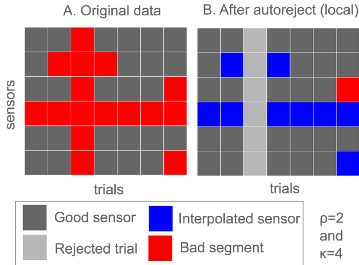
Figure 4.5: Segments of the epochs are either interpolated or the whole epoch is rejected, based on the parameter k (if there are more than k bad segments, reject the whole epoch) and \rho (interpolate \rho worst epochs). Figure taken from [75].
