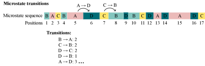
Figure 4.12: Transitions of the states within a microstate sequence.
