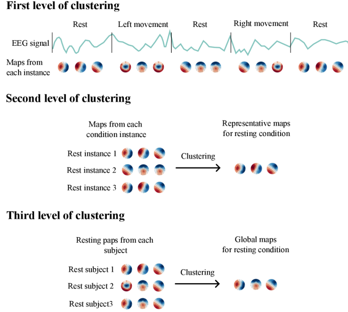
Figure 4.7: Levels of clustering in the process of microstate extraction.
