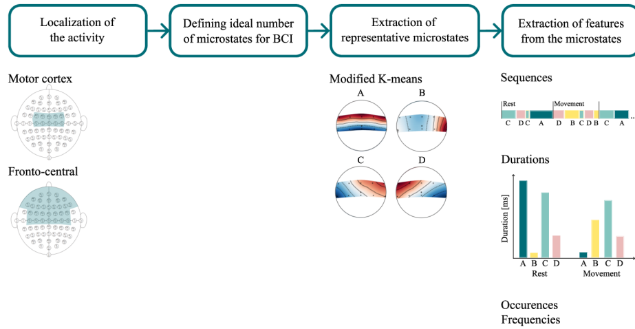
Figure 4.2: Proposed pipeline for the microstate analysis for the BCI application.
