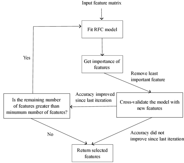
Figure 4.15: Recursive feature elimination with cross-validation.
