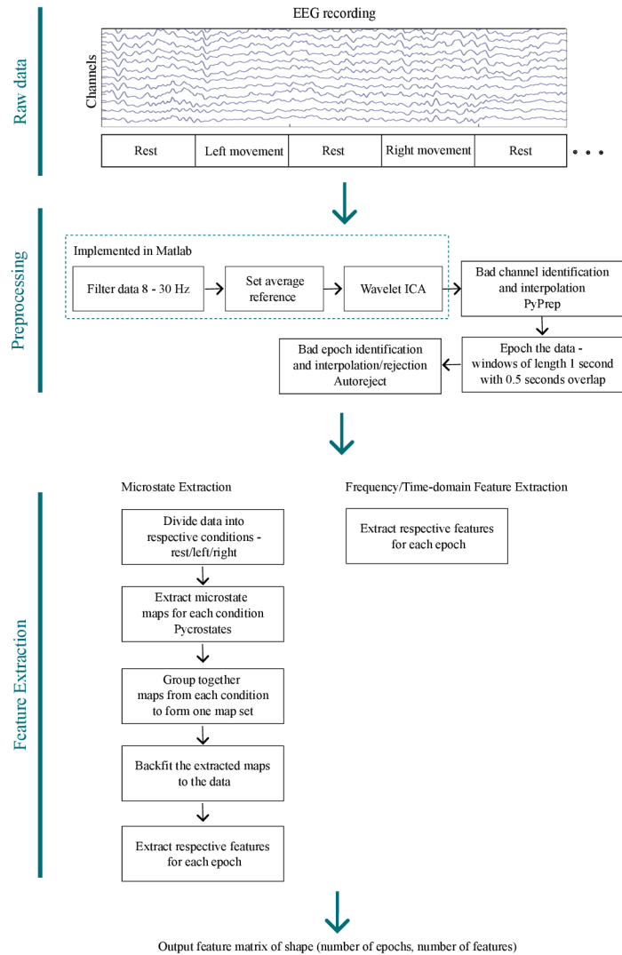
Figure 5.1: Implemented pipeline of the data preprocessing and feature extraction.
