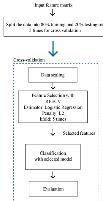
Figure 5.3: Implemented pipeline of the feature selection and cross validation.
