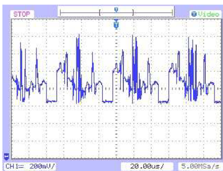
Obr. 38 R/CIN_ENC
