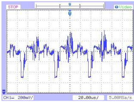
Obr. 35 Y/CVBSIN_ENC
