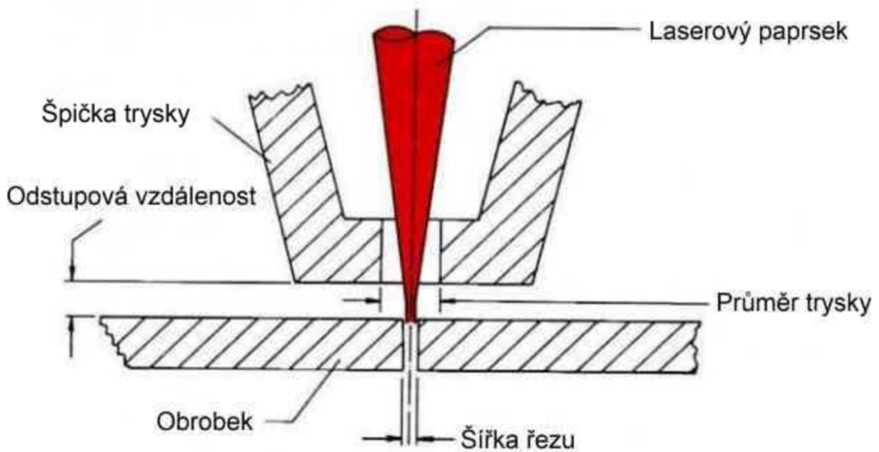
Obr. 6 Geometrie trysky [17].
