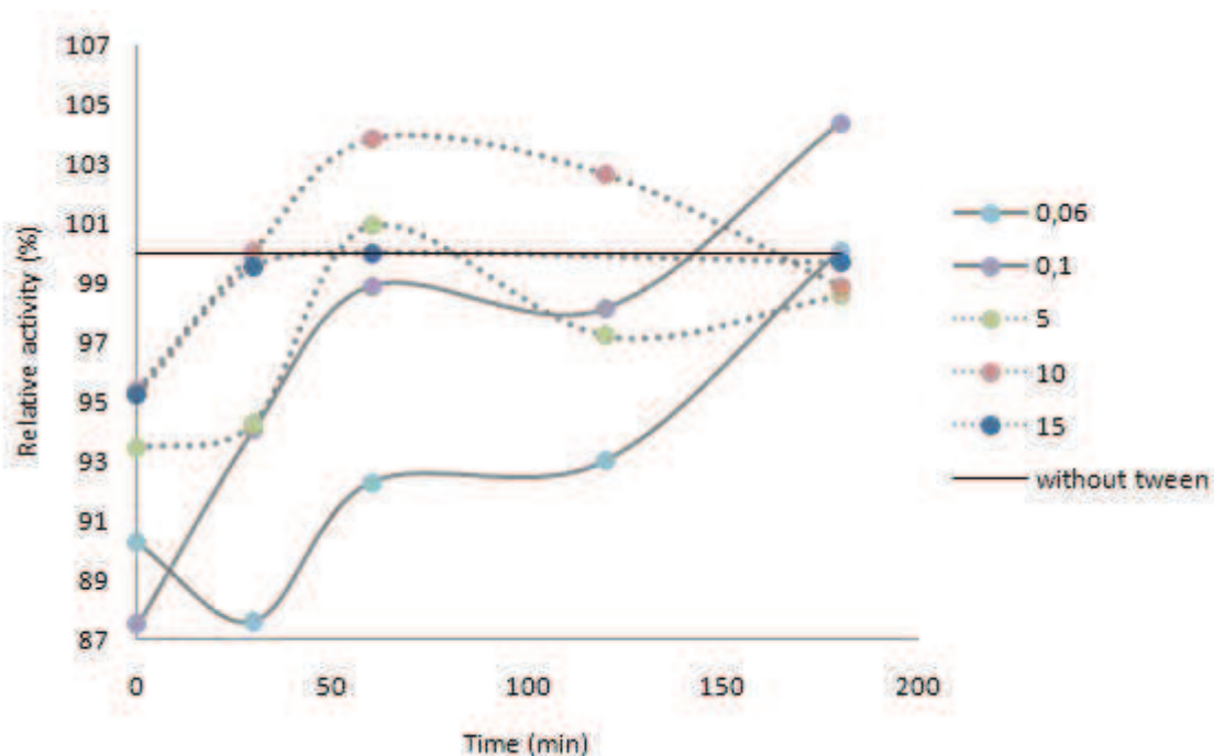
Figure 22 Incubation of RA in phosphate buffer solution with tween 20, RA lipase specific activity before incubation with tween was 9.9 \text{ U}\cdot\text{mg}^{-1}
