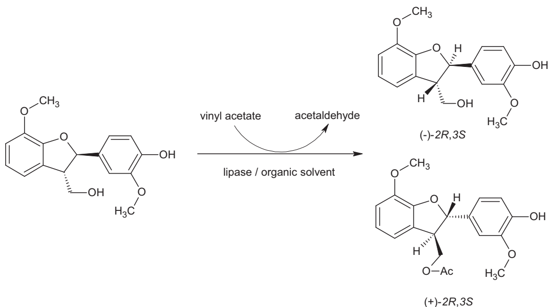
Figure 6 Lipase catalysed acylation of (\pm) -trans-2-(4-hydroxy-3-methoxyphenyl)-3-hydroxymethyl-7-methoxy-2,3-dihydroxybenzo[b]furan [20].
