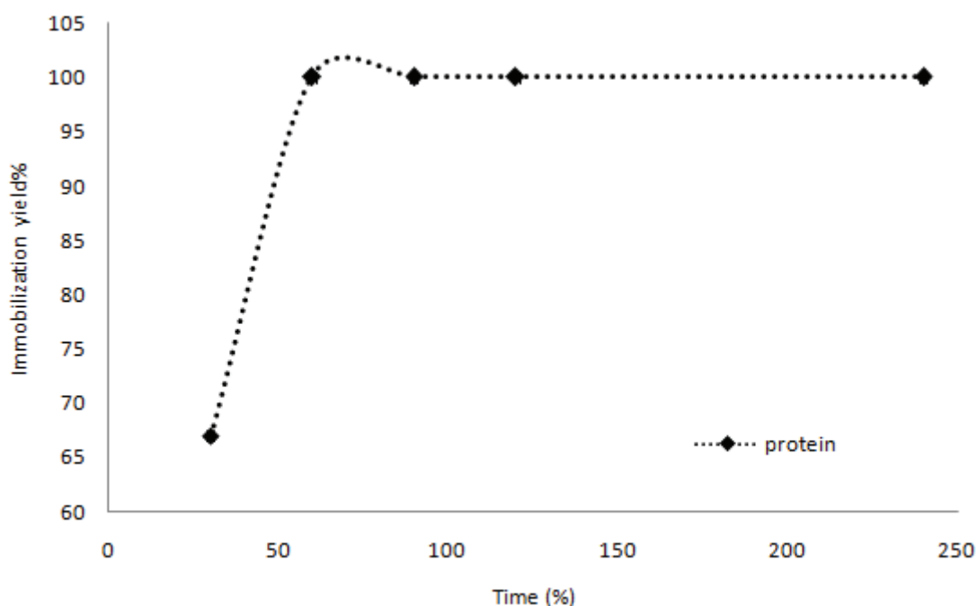
Figure 25 The influence of incubation time from 30 to 240 min on coupling and immobilization yield of RA lipase immobilized on carbon-based carrier treated with tween 20 (110 \mu\text{l} )
