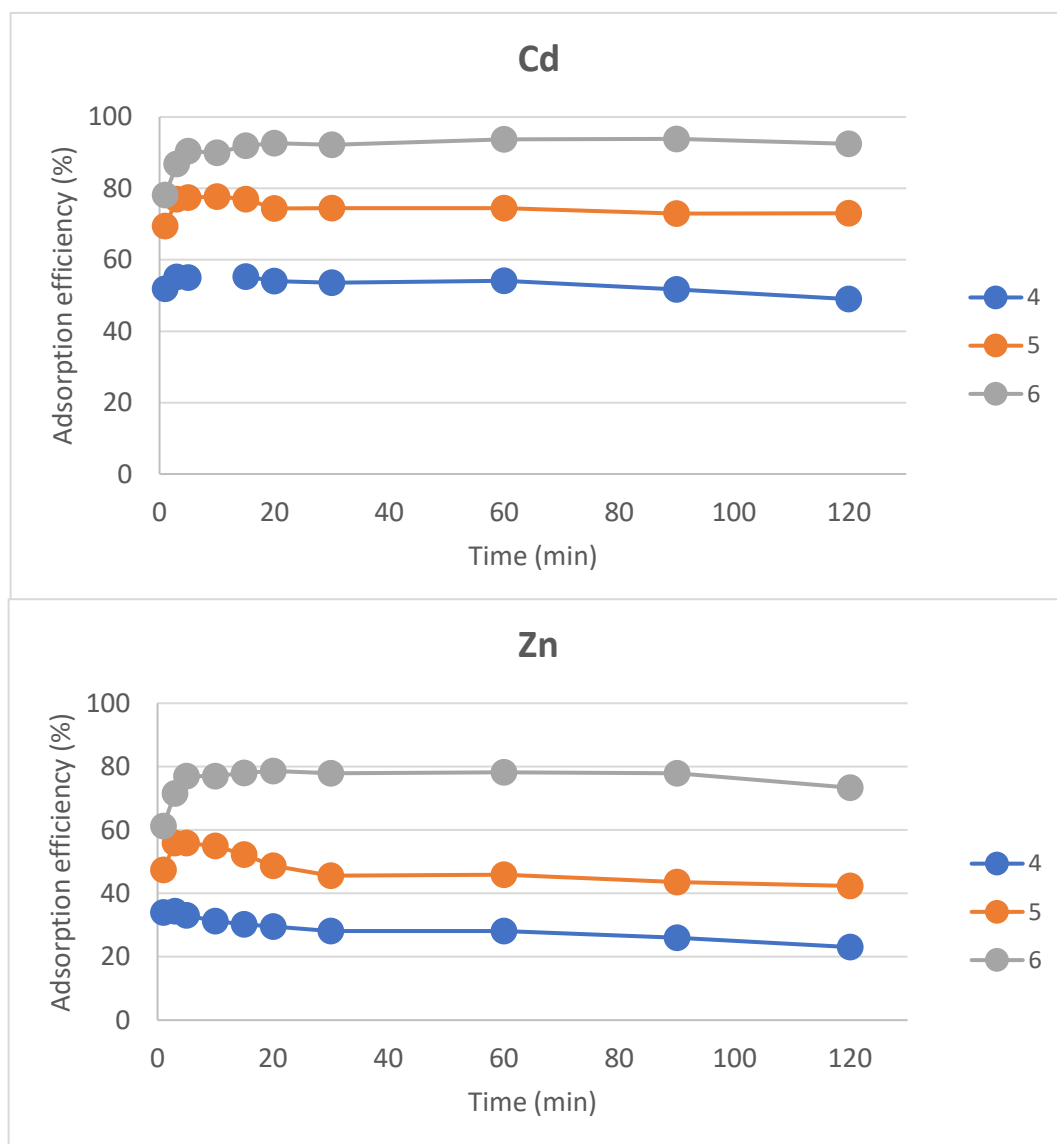
Figure 8. Co-adsorption kinetic experiment of Cd and Zn using AMO/BC at controlled pH 4, 5 and 6.
