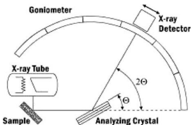
Figure 1. Figure 1. Schematic diagram of a diffractometer system (Bunaciu Andrei A et al., 2015).
