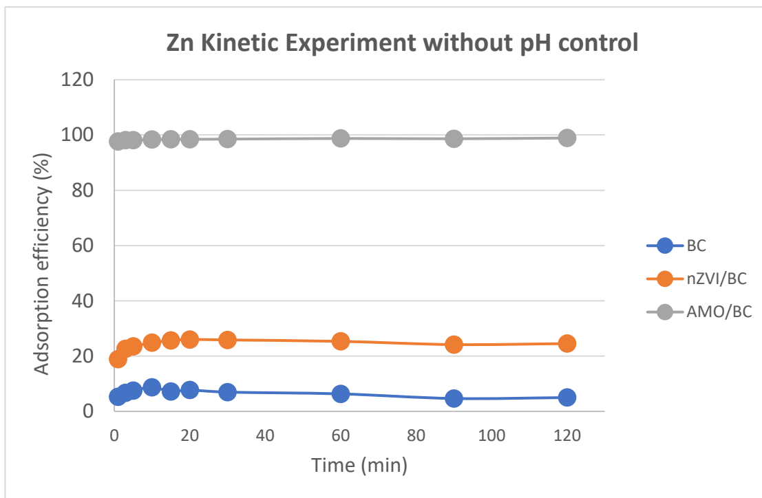
Figure 5. Kinetic experiment of Zn using BC, nZVI/BC, and AMO/BC without pH control.
