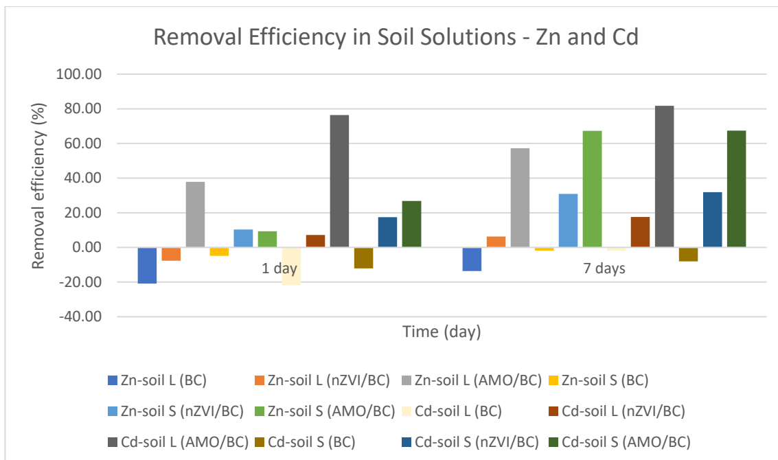
Figure 21. Removal Efficiency in soil L and soil S solutions using BC, nZVI/BC, and AMO/BC for Zn and Cd.
