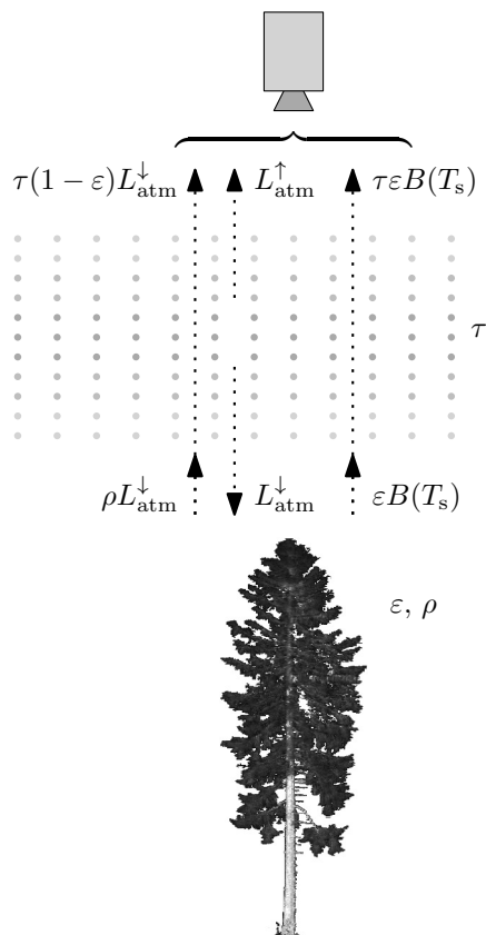
Figure 2.4: The radiance incident to the sensor in the thermal region originates mainly from three sources: 1) radiance \tau\varepsilon B(T_s) emitted by an object; 2) reflected downwelling atmospheric radiance \tau(1 - \varepsilon)L_{atm}^\downarrow ; 3) upwelling atmospheric radiance L_{atm}^\uparrow emitted by the atmosphere itself.
