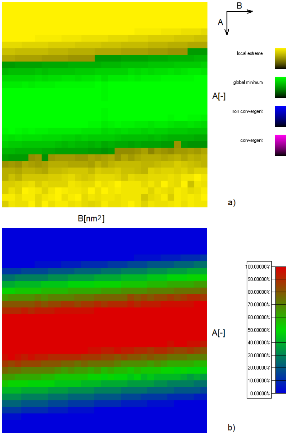
Figure 53: An example of \mathbf{B}^P of 500nm thick \text{Si}_3\text{N}_4 film on silicon substrate when all coefficients were unfixed and where the thickness d was omitted.
