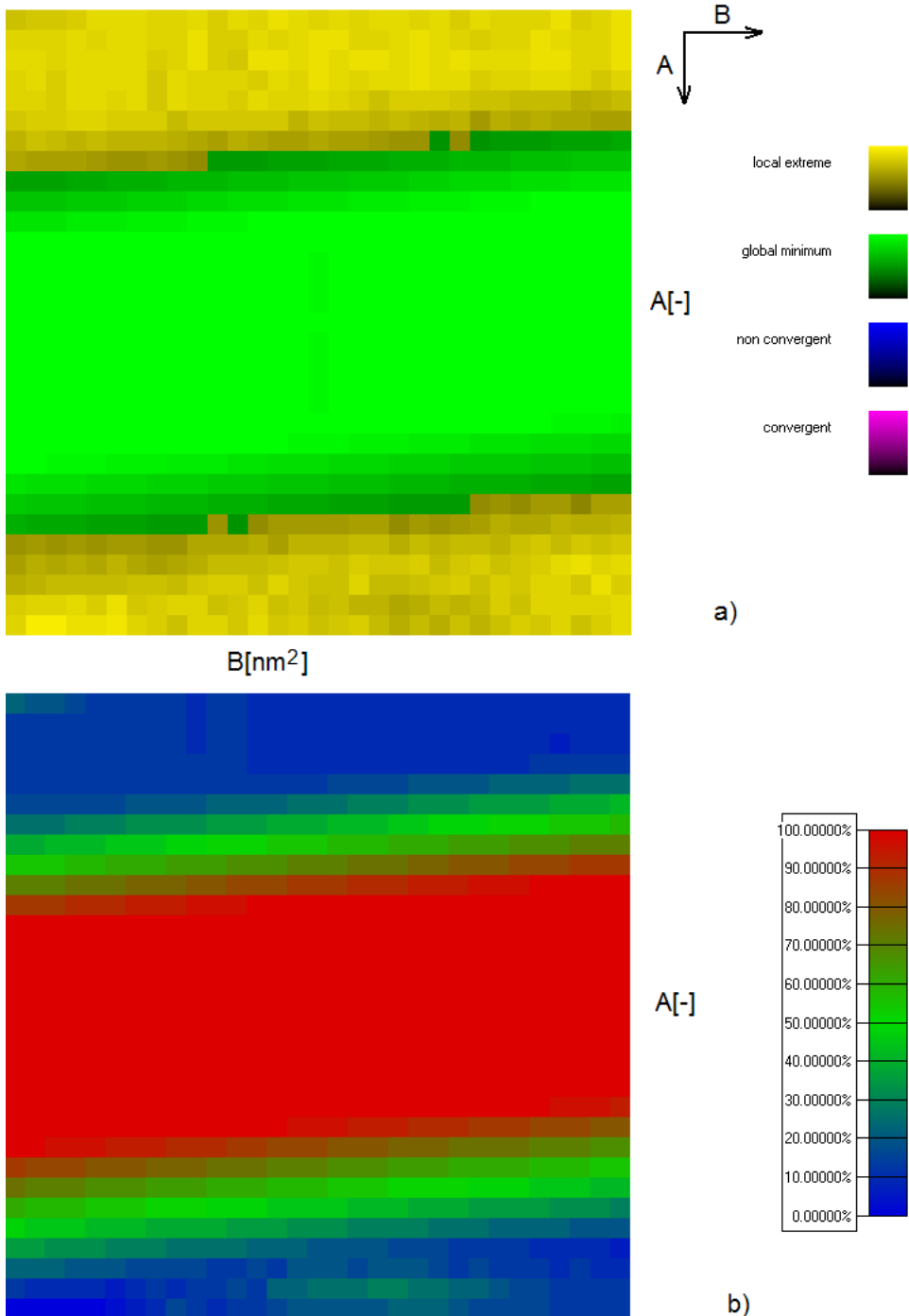
Figure 49: An example of \mathbf{B}^P of 460nm thick PMMA film on silicon substrate when all coefficients were unfixed and where the thickness d was omitted.
