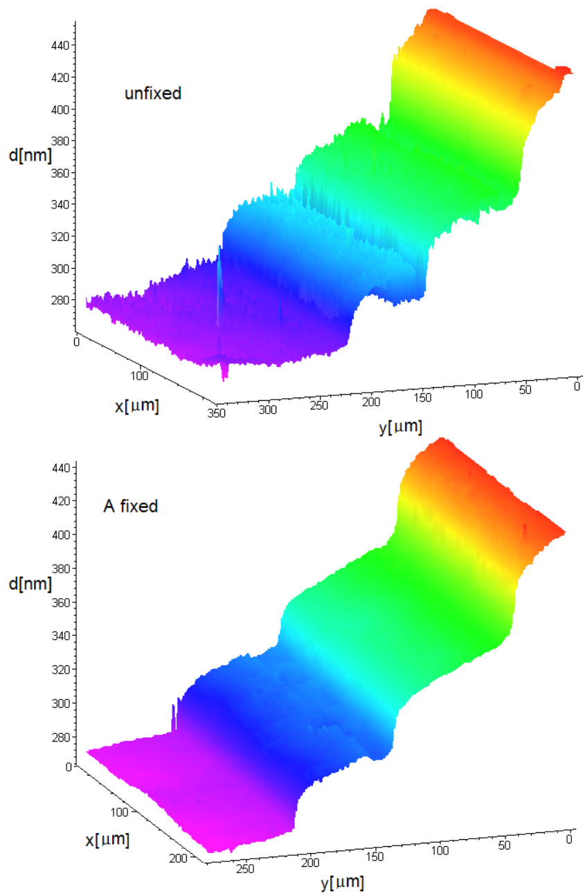
Figure 30: The example of the measurement of SiO 2 film characteristics with and without fixing the coefficients.
