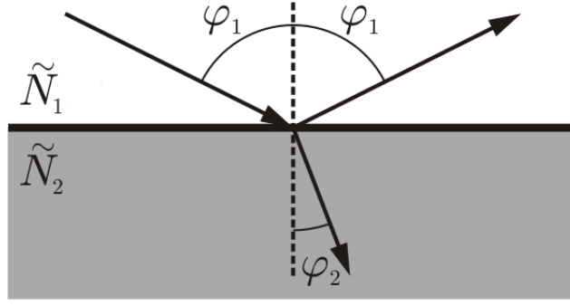
Figure 3: Light reflection at interface of two different optical media.
