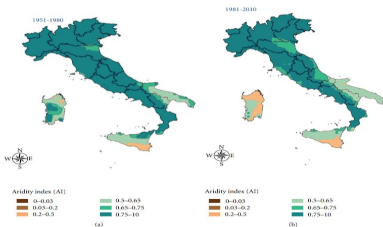
FIGURE 3: The spatial distribution of the Aridity Index in Italy by time period.
