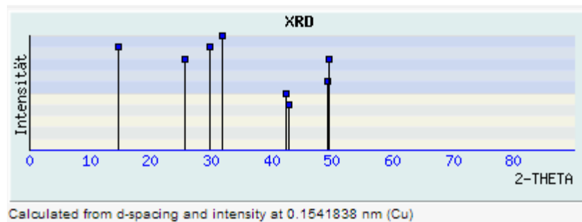
Obr. 10: Rentgenogram Bassanitu
