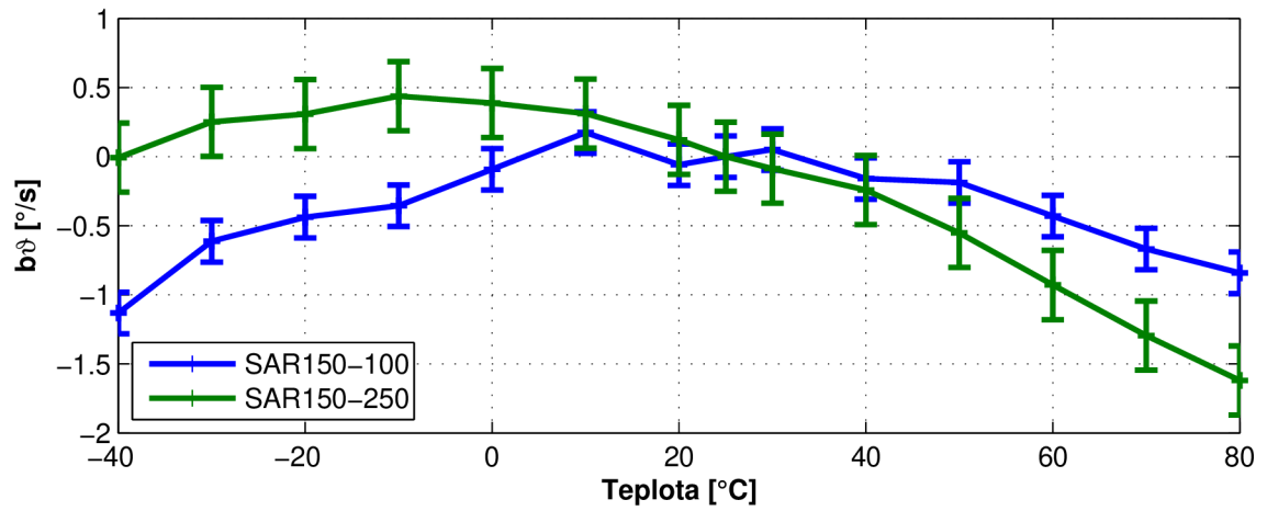
Obr. A.19: Teplota: posun nuly (SAR150-100, SAR150-250)
