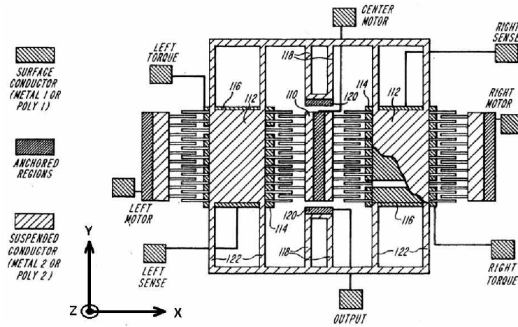
Obr. 2.8: Draper Tuning Fork Gyroscope [13]
