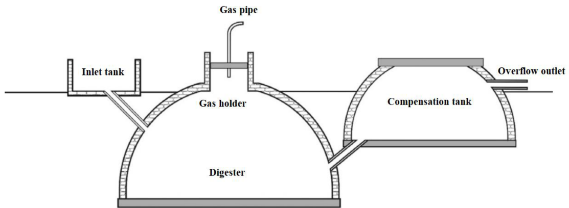
Figure 6. Biogas digester scheme (fixed-dome type) (Roubik et al. 2020).
