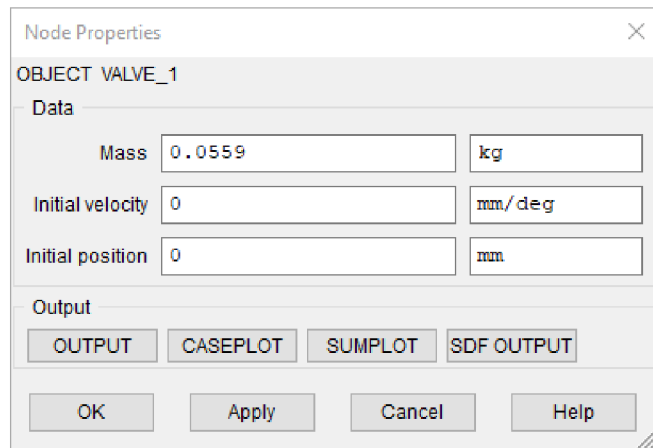
Obr. 5.27: Definice ventilu
