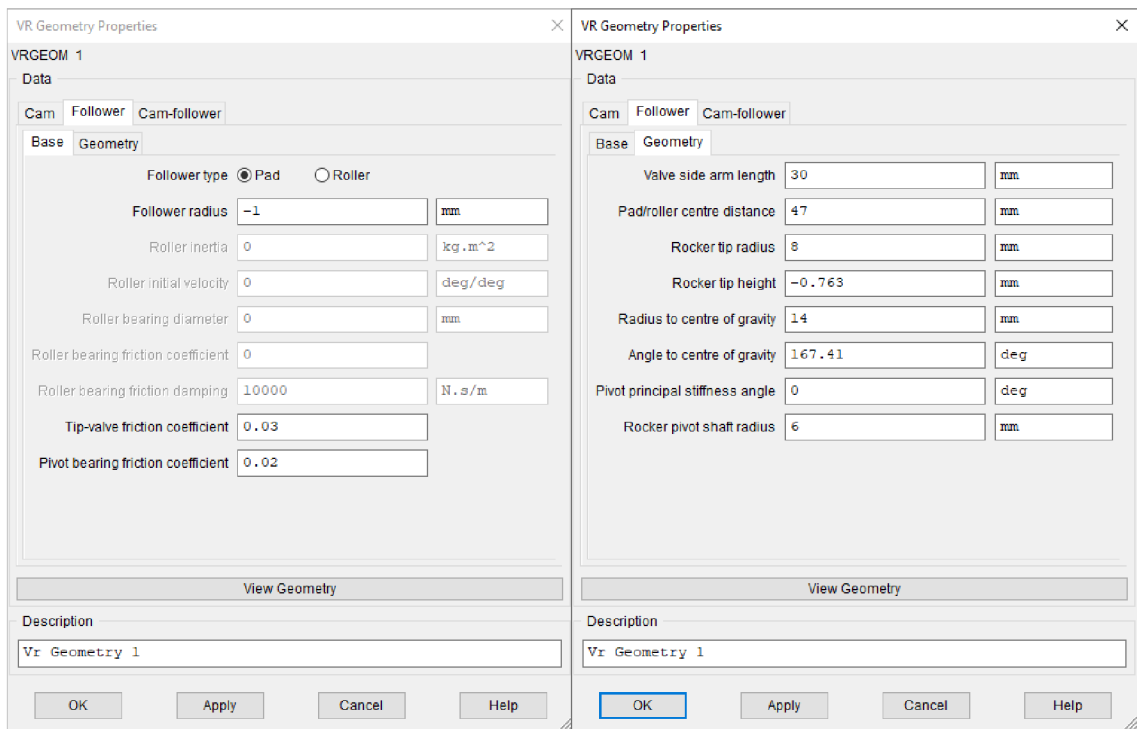
Obr. 5.40: Definice vahadla
