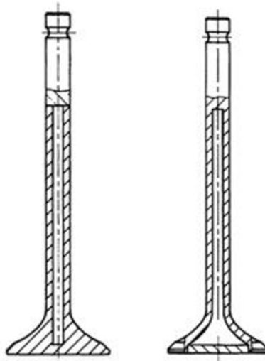
Obr. 2.11: Duté ventily [4]
