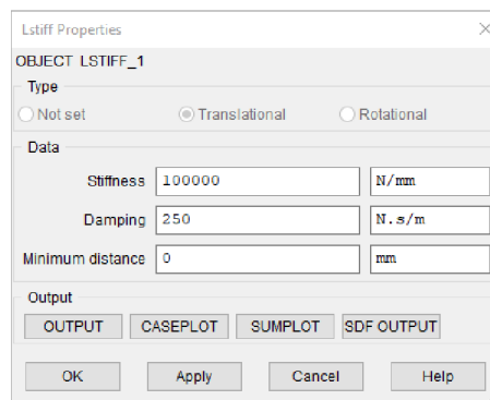
Obr. 5.22: Definice tuhosti
