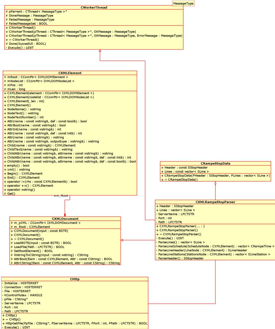
Figure 8.5: XML
