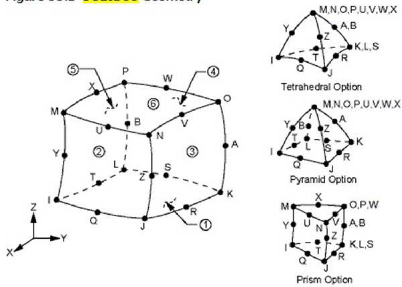
Obr. 30 Element Solid95
