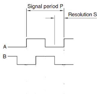
Incremental* 2 channels A and B in quadrature (90° phase shifted)
