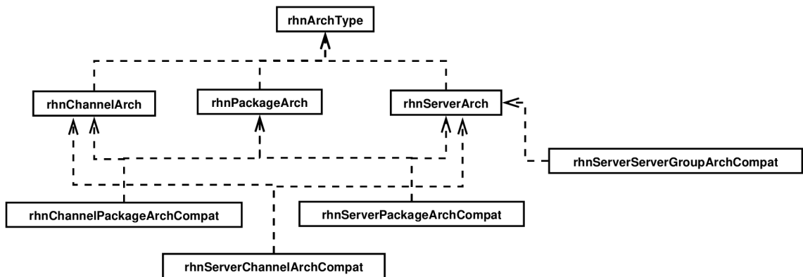
Figure 5.1: The connection between sql tables
