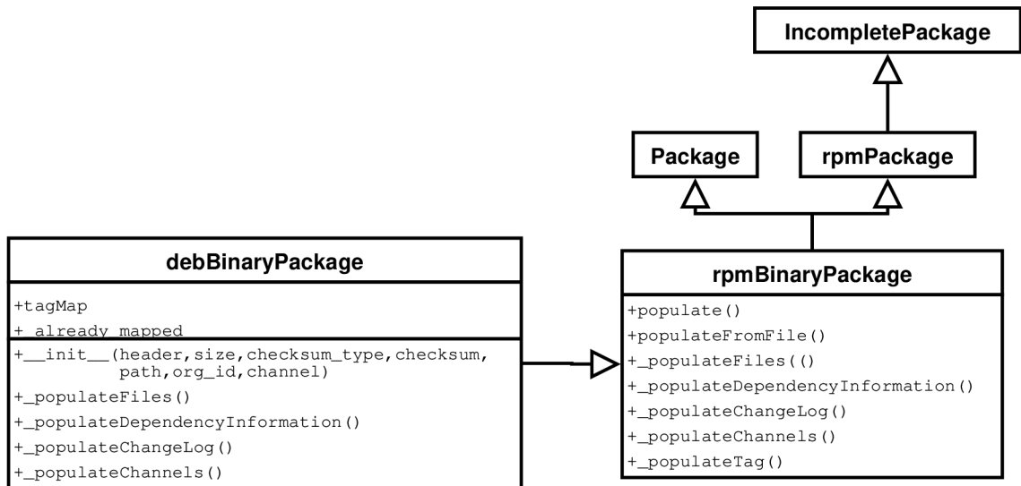
Figure 6.1: The class diagram for debBinaryPackage
