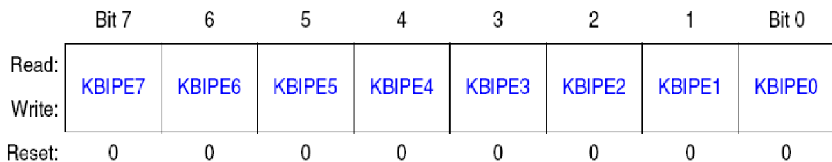
Obr. 7.7: KBI Pin Enable Register (KBI1PE)
