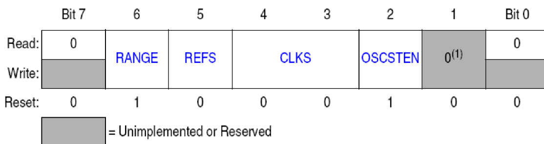
Obr. 7.1 ICG Control Register 1 (ICGC1)
