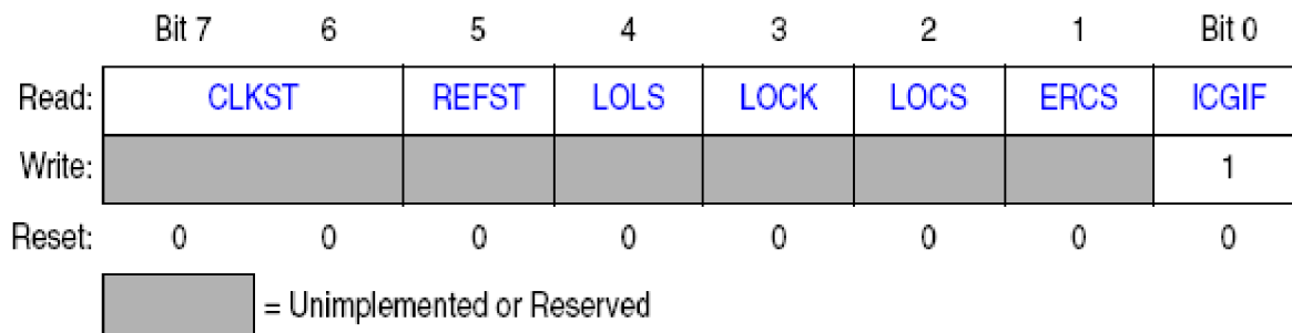
Obr. 7.2: ICG Status Register 1 (ICGS1)
