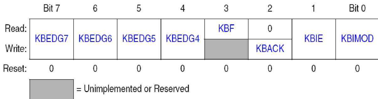
Obr. 7.6: KBI Status and Control Register (KBIISC)
