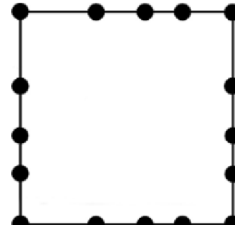
(l) CoP-Tag [73], 2012
