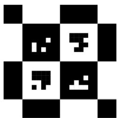
(e) CALTag [61], 2010
