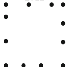
(n) Pi-Tag [70], 2013
