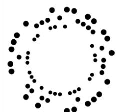
(i) RUNE-Tag [68], 2011
