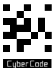
(e) CyberCode [30], 2000
