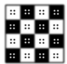
(k) BlurTags [72], 2012
