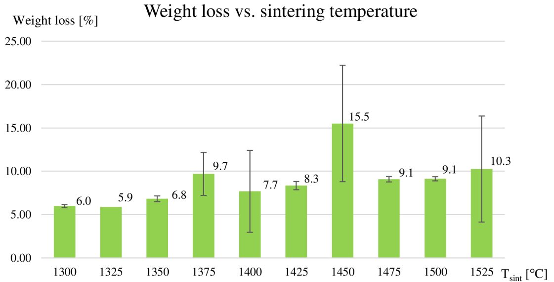
Fig. 5.4 Plot of dependence of weight losses on sintering temperature.
