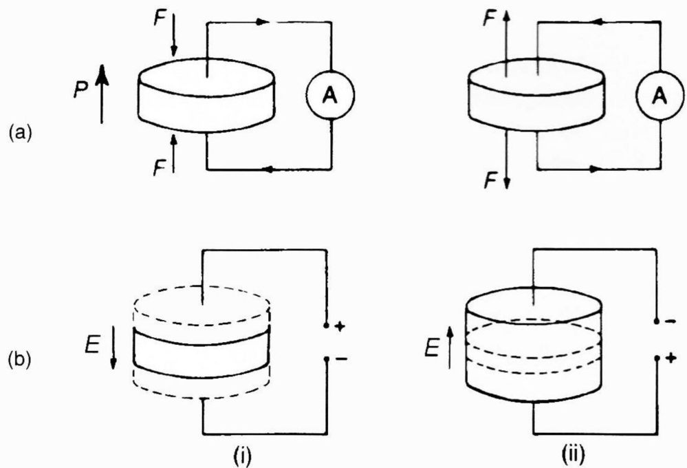
Fig. 2.1 (a) The direct and (b) inverse piezoelectric effect: (i) contraction; (ii) expansion. The broken lines indicate the original dimensions. [1]
