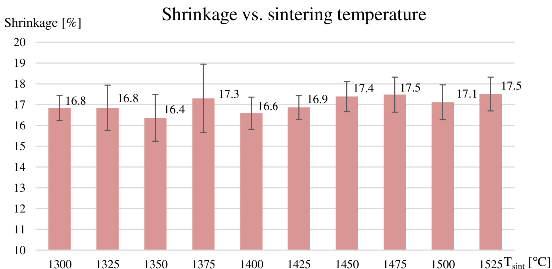
Fig. 5.3 Plot of dependence of shrinkage on sintering temperature.
