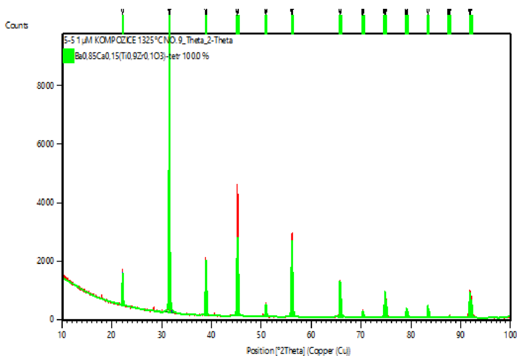
Fig. 5.1 The XRD trace for sintering temperature 1325 °C.
