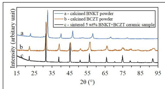
Fig. 3. XRD patterns of the calcined BNKT and BCZT powders, and the 5 wt% BNKT+BCZT ceramic sample sintered at 1500 °C.
