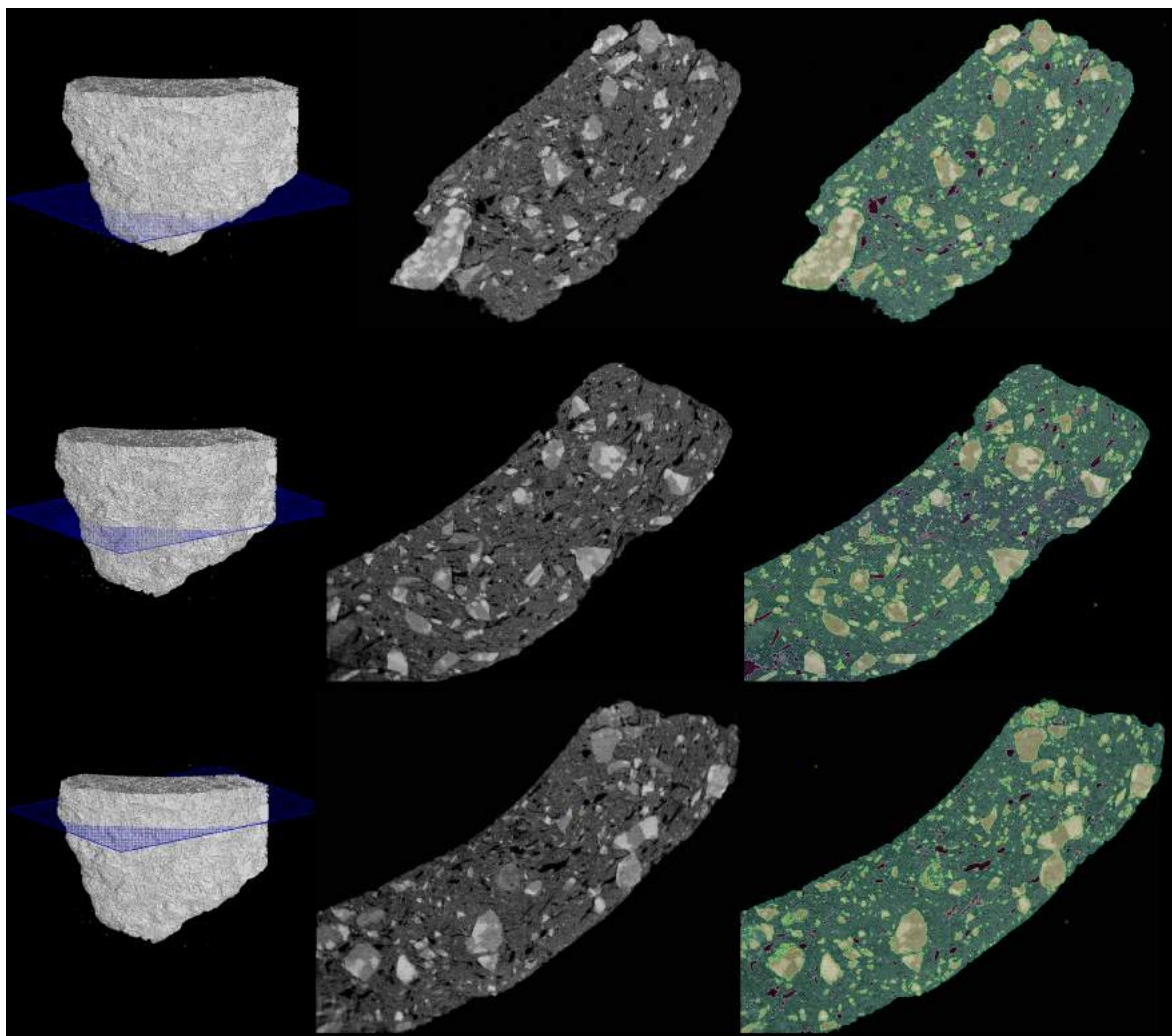
Fig. 4.6: Left: 3D model of a selected sample; Middle: Virtual cross-section, position of the slice is indicated by the blue plane in the 3D model; Right: Segmentation of different pottery components of the sample. Green-clay, yellow-inclusions, purple-voids.
