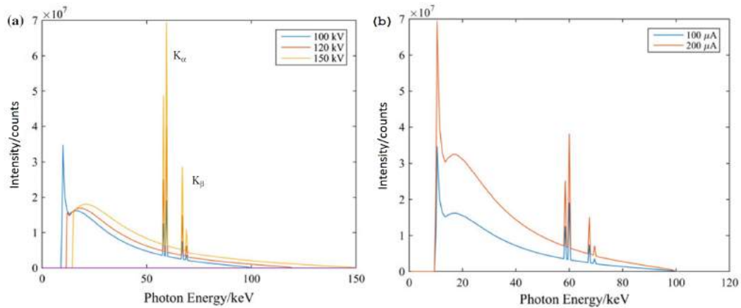
Fig. 1.4: X-ray spectrum at; (a) 100, 120 and 150 kV, (b) 100 and 200 \mu\text{A} for a tungsten target. X-ray spectra were obtained by software SpekCalc [8].
