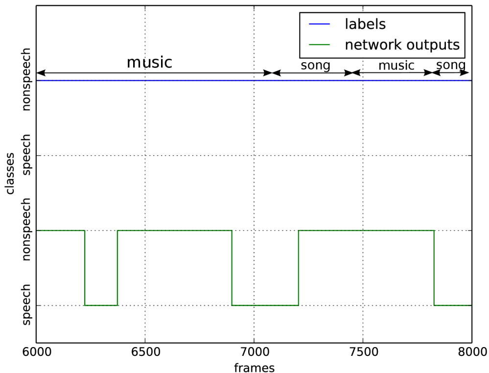
Figure 3.5: An example of comparison between labels and network outputs of the speech detection in a 20 seconds long passage from a radio recording. Whole passage consists of music with singing sequences.
