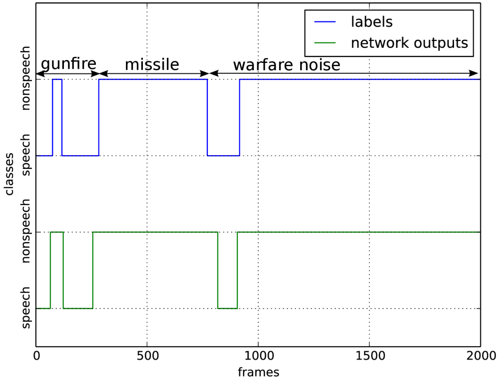
Figure 3.4: An example of comparison between labels and network outputs of the speech detection in a 20 seconds long passage from a warfare footage. This recording includes gunfire, launch of missile and more warfare noise. The results for this input are: FAcc 89.57%, hit rate 8.11% and BAcc -78.38%.
