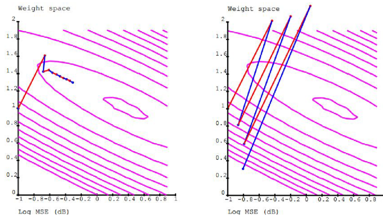
Figure 2.9: An example of a gradient descent in order to adequately (left) and too high (right) set learning rate [13].
