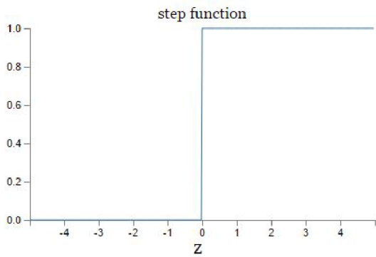
Figure 2.7: Graphs of a step function
