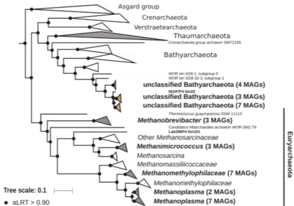
Figure 5 Phylogenomic tree of the archaeal domain. This maximum-likelihood tree was inferred from a concatenated alignment of 43 proteins (6,682 positions) using the LG+G+I+F model of amino-acid evolution. Branch supports were calculated using a Chi 2 -based parametric approximate likelihood-ratio test. Names in bold included MAGs recovered in the present study. Clusters shaded in brown consist exclusively of MAGs from termite guts and clusters shaded in gray contain genomes from termite guts. The Asgard group was used as outgroup. Full-size DOI: 10.7717/peerj.8614/fig-5
