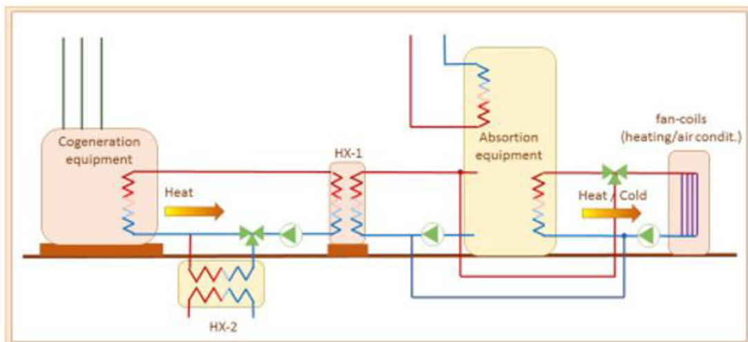
Figure 6: Tri-generation installation scheme (Sala Lizarraga & Picallo-Perez, 2020)
