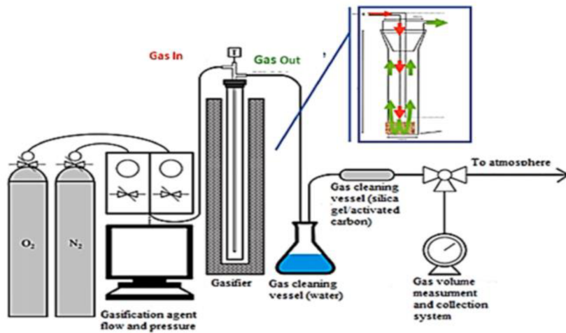
Figure 10: Schematic representation of the laboratory gasification system (Vaskalis, et al., 2019)
