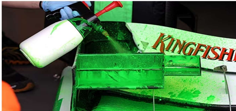
Obr. 26 Nanášanie Flow-vis [35]
