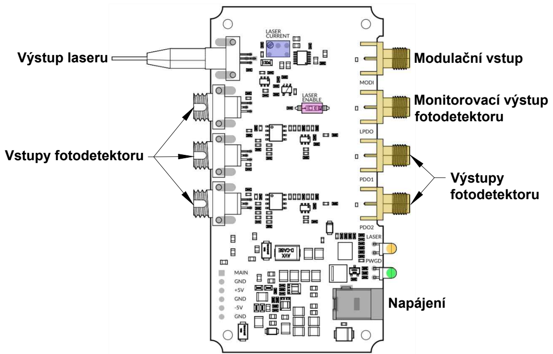
Obr. 6.5: Koheron LPD100 [20].
