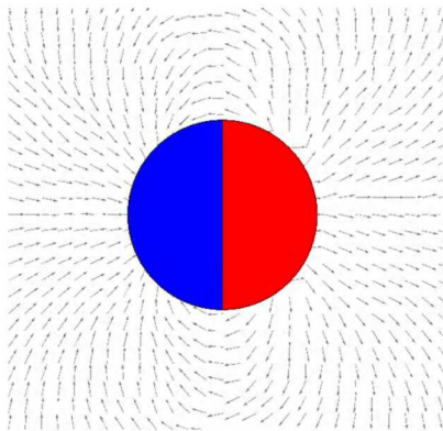
Fig. 1.14: Diametric magnet [32]
