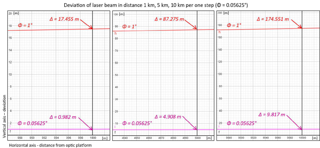
Fig. 4.13: Deviation \Delta of the laser beam in distances 1 km, 5 km, and 10 km on a current prototype for micro-step size 0.05625^\circ . For comparison, red beam is a theoretical beam with a step size of 1^\circ .
