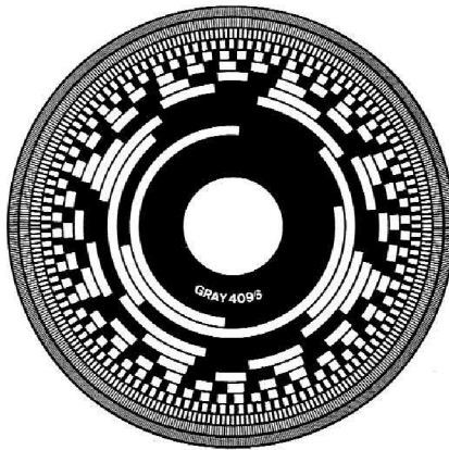
Fig. 1.9: 12bit Absolute optical encoder with gray code [22]
