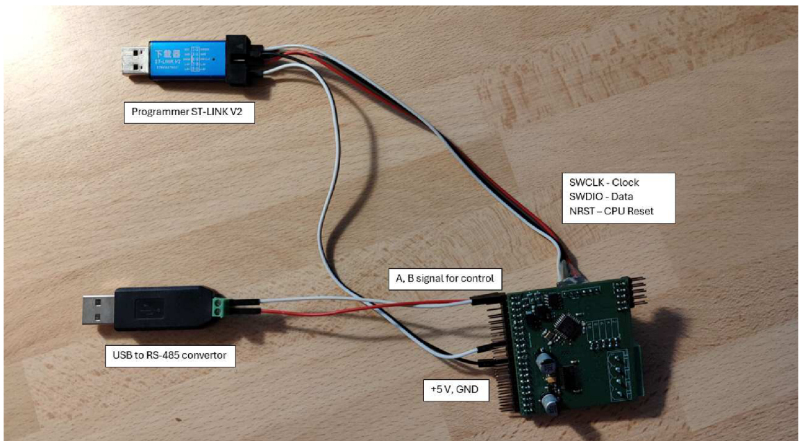
Fig. 4.21: Standalone implementation
