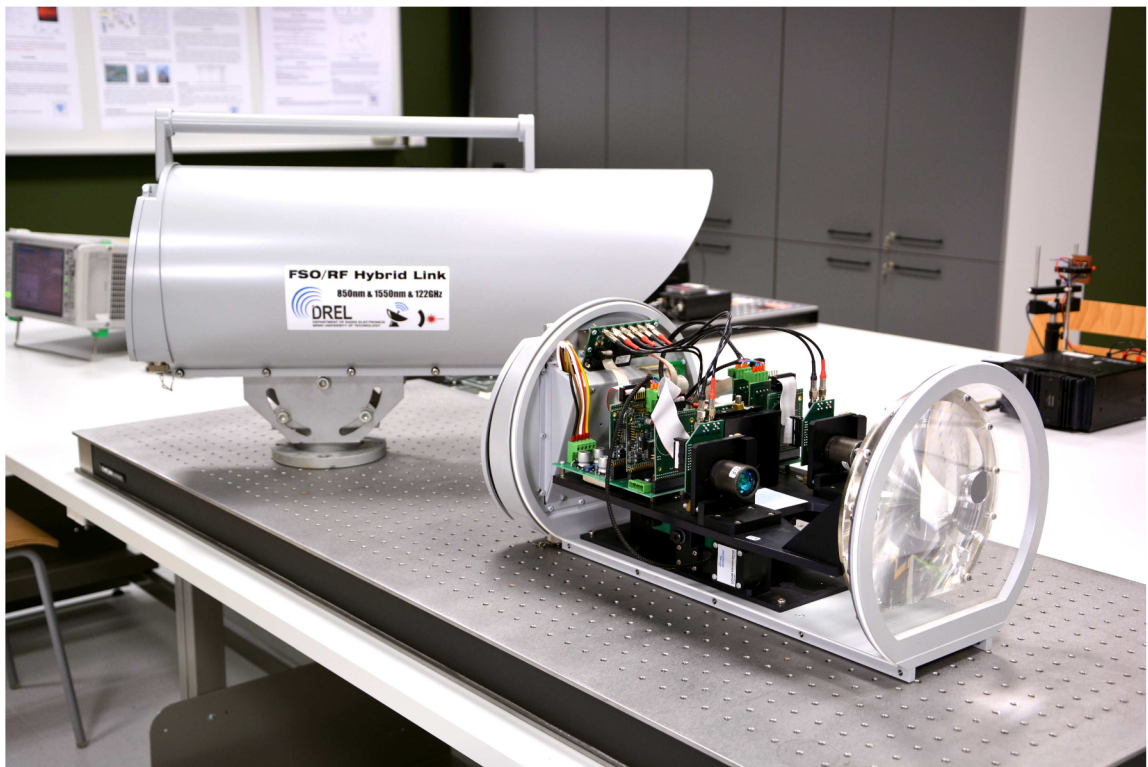
Fig. 3.1: Opto-mechanical platform
