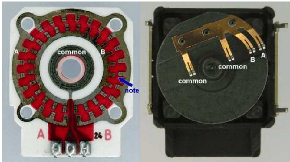
Fig. 1.6: Incremental contact encoder disc [18]
