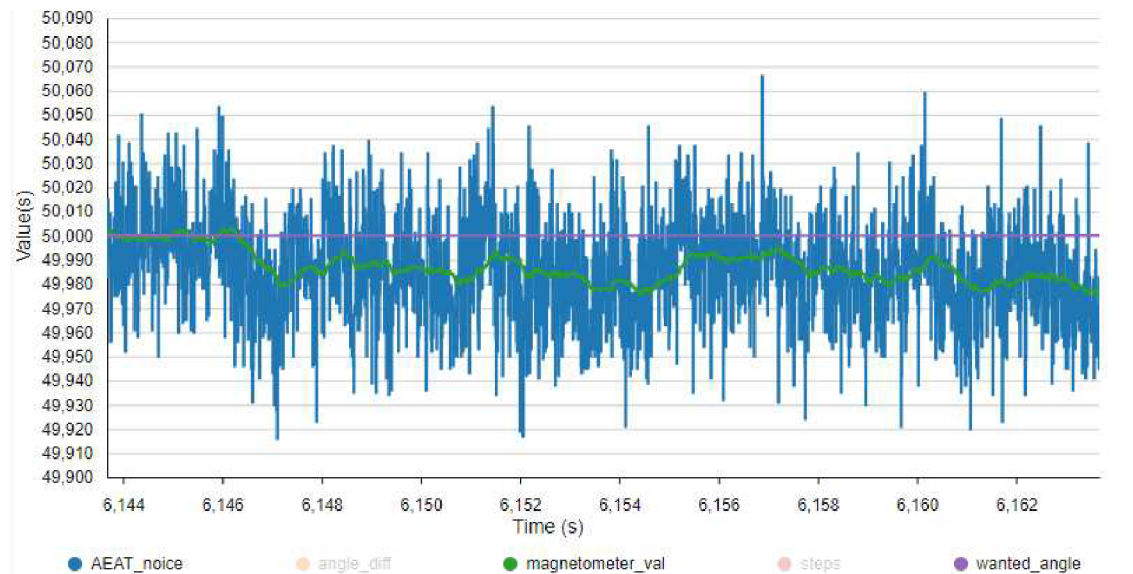
Fig. 4.26: Filtred value green , noise from sensor blue and wanted angle purple . On the vertical axis is angle in ( ^{\circ} )
