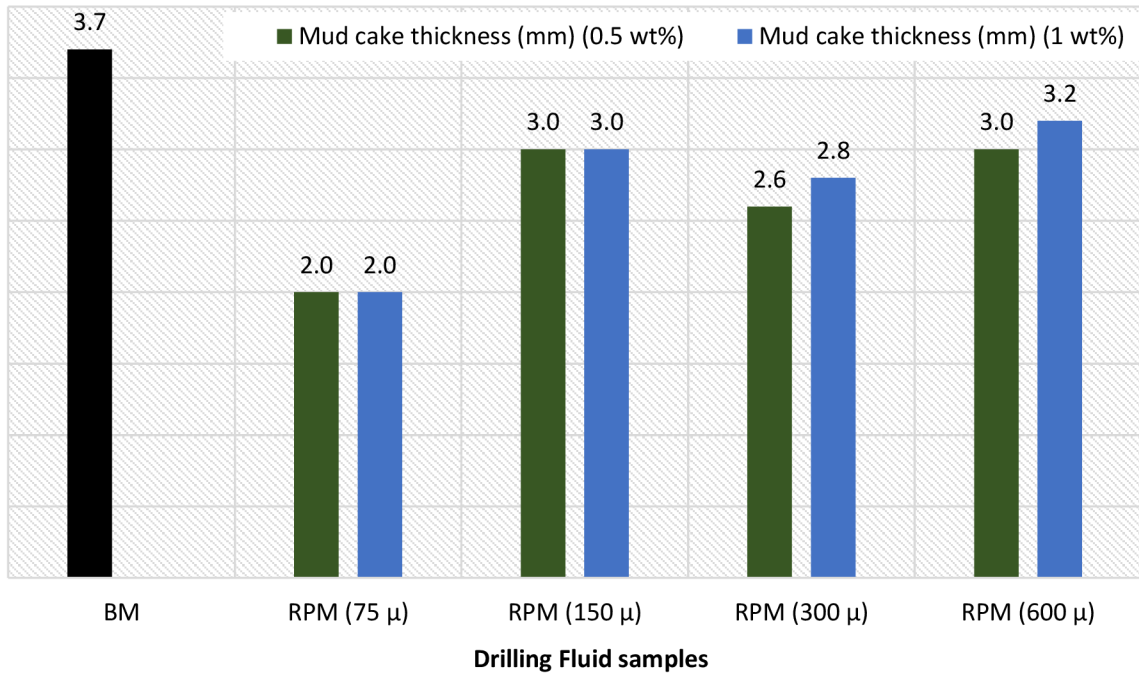
Figure 21 The results of mud cake thickness of rambutan peels powder different particle size vs different concentrations
