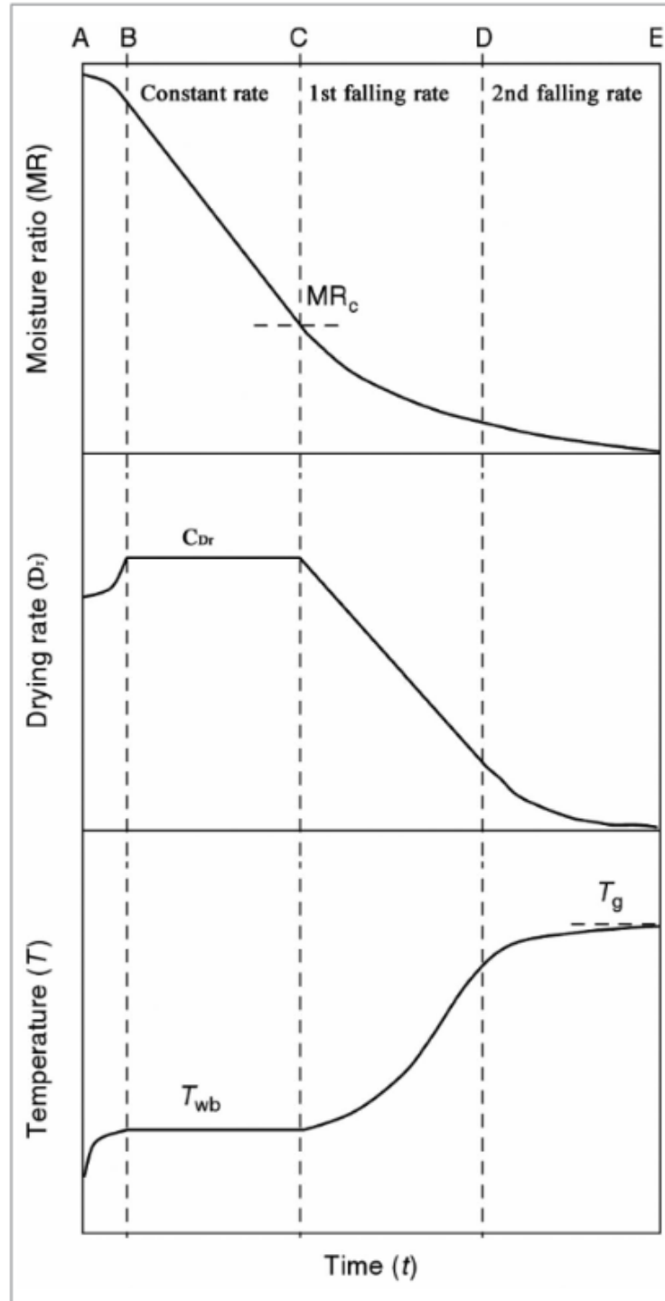
Figure 5. A typical drying curve of agricultural products showing constant rate and falling rate periods (Onwude et al. 2016; Carrin and Crapiste, 2008).
