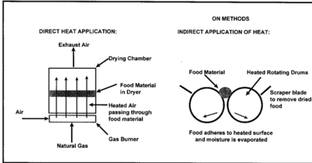
Figure 1. Diagram of direct and indirect heated air.
