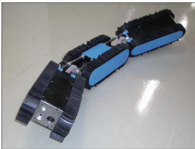
Obr. 15 Souryu-IV [8]
