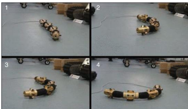
Obr. 12 ACM-S1 [8]
