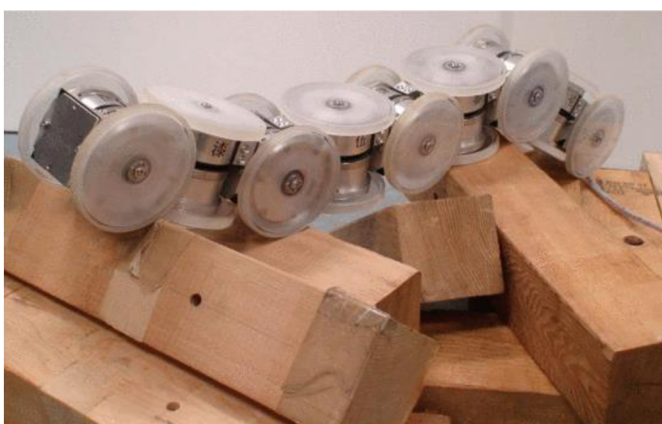
Obr. 13 ACM-R4.1 [15]
