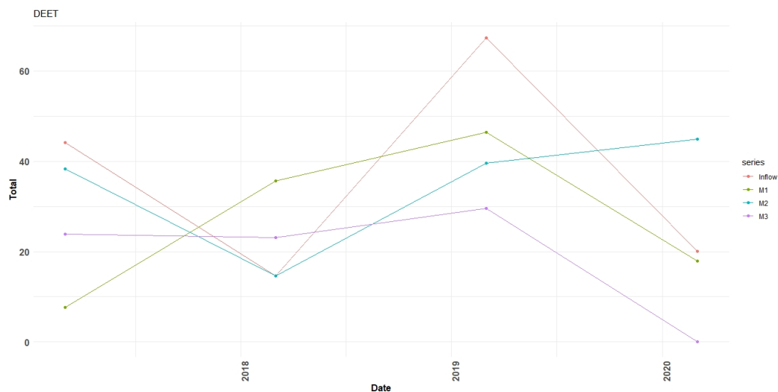
FIGURE 6.3: DEET
