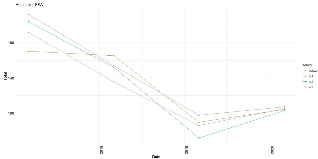
FIGURE 6.2: Acetochlor ESA
