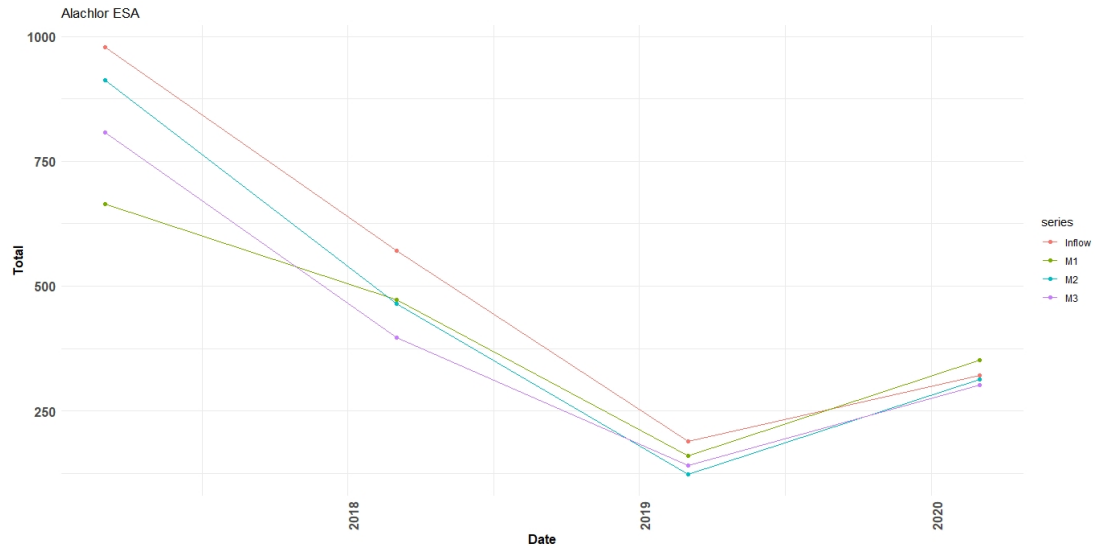
FIGURE 6.1: Alachlor ESA
