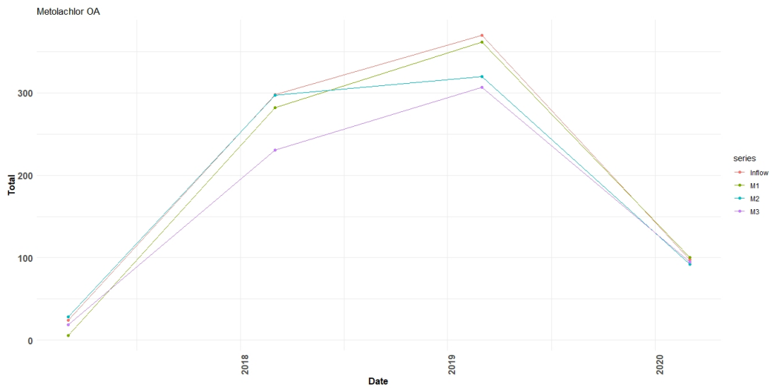
FIGURE 6.8: Metolachlor OA
