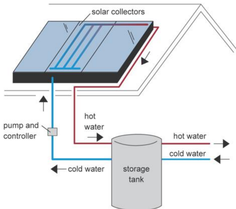
Figure 3. Basic components of a solar water heating system [20]
