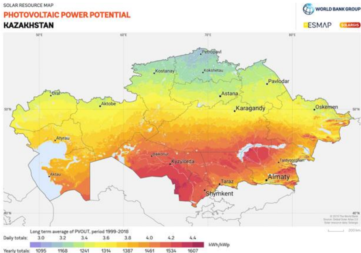
Figure 5. Solar resource map of Kazakhstan [43]
