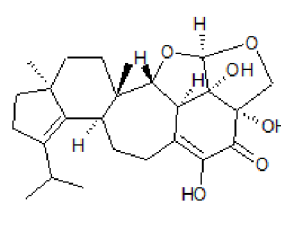
Erinacin S
