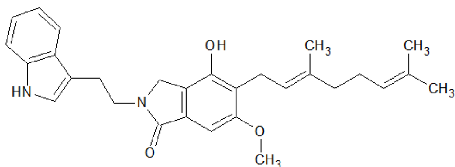
Korallocin C
