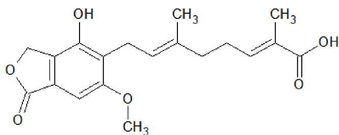
Korallocin A
