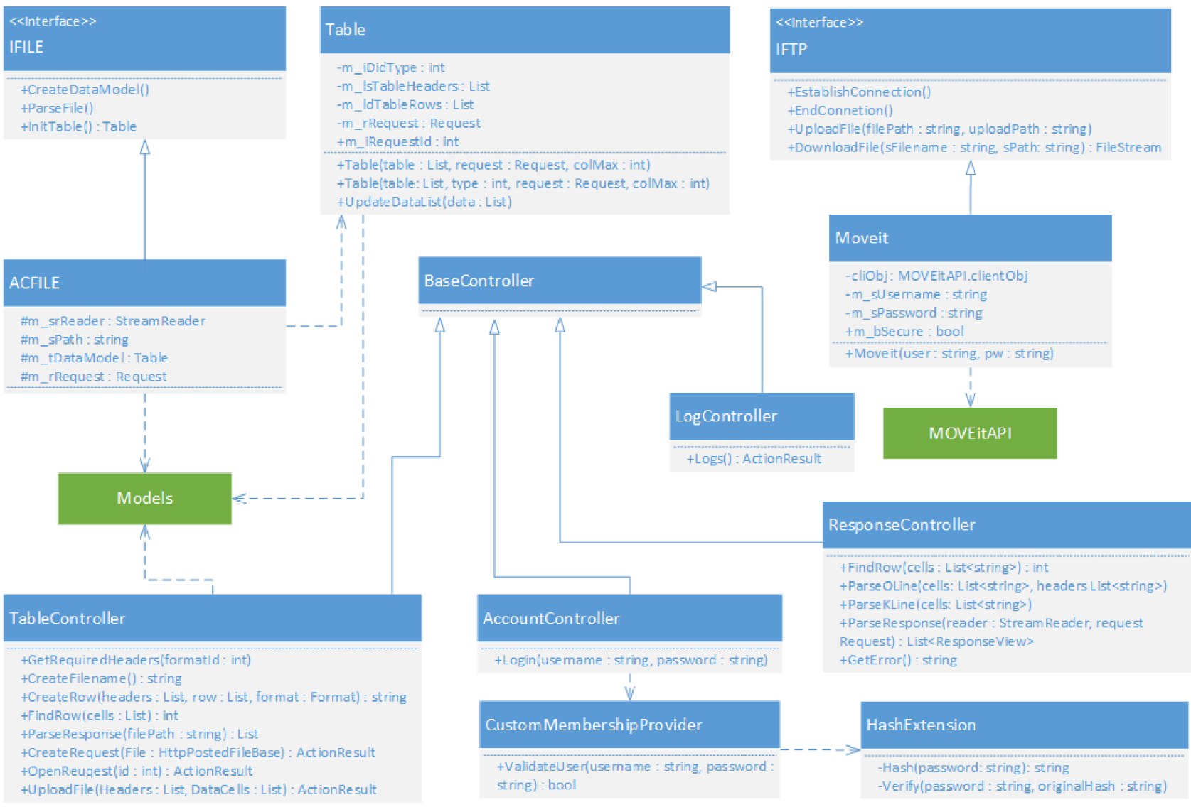
Picture A.1: Class diagram describing structure of the ASP.NET application
