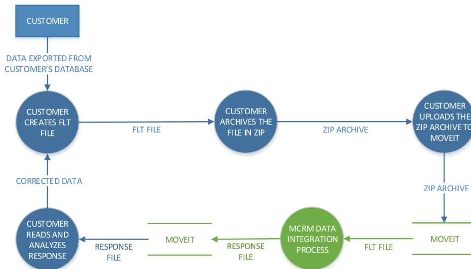
Picture 3: Data integration process from customer's perspective
