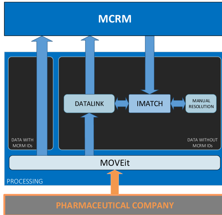
Picture 1: Simplified MCRM identifier mapping process
