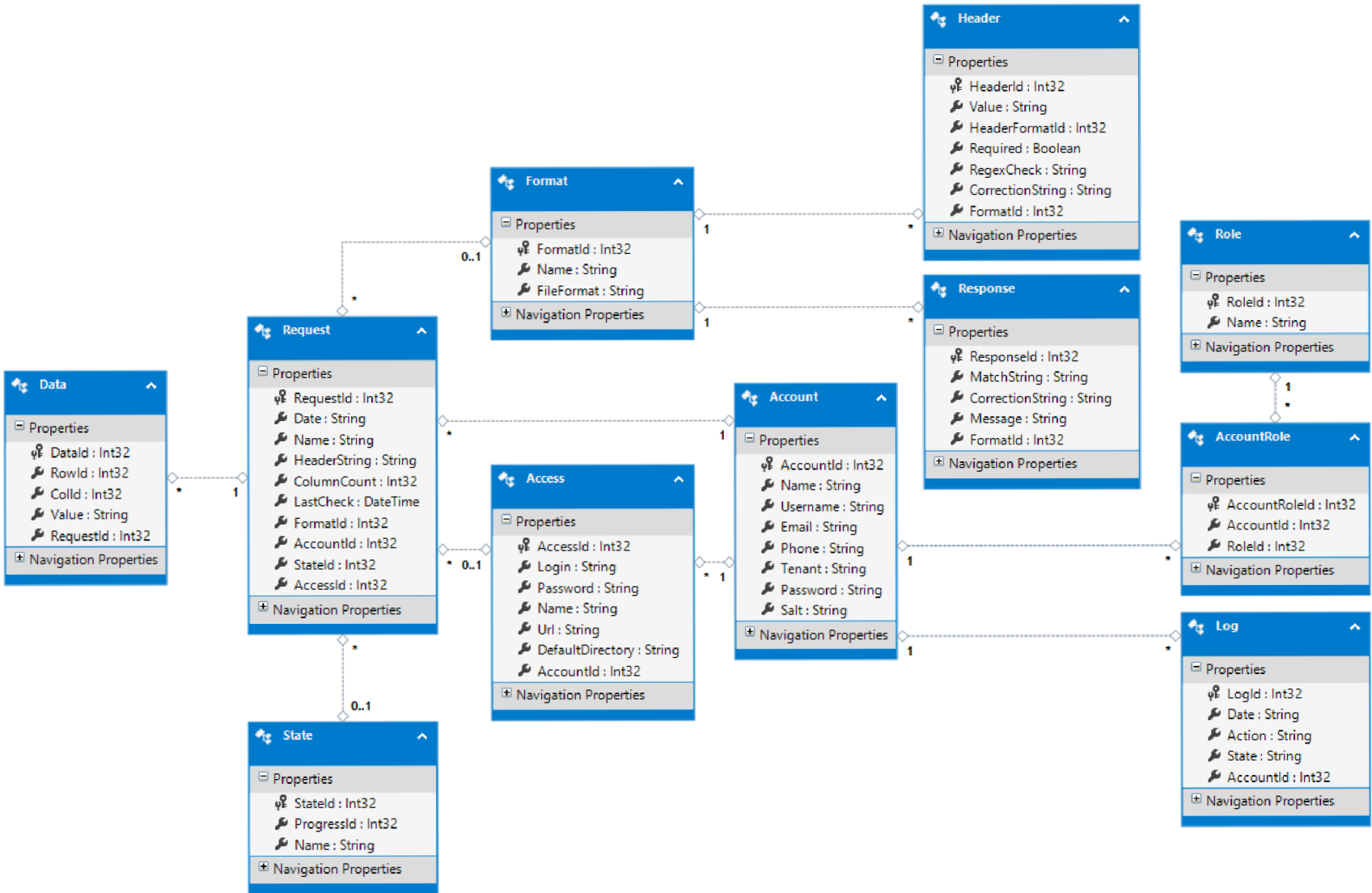
Picture A.2: ASP.NET application database ER diagram
