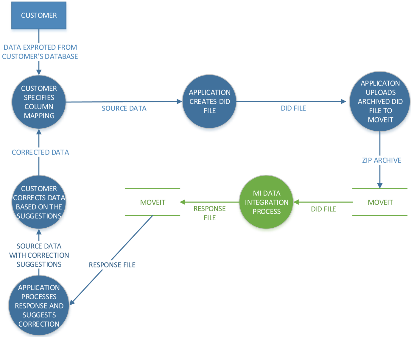
Picture A.4: Data integration process from customer's perspective with the application
